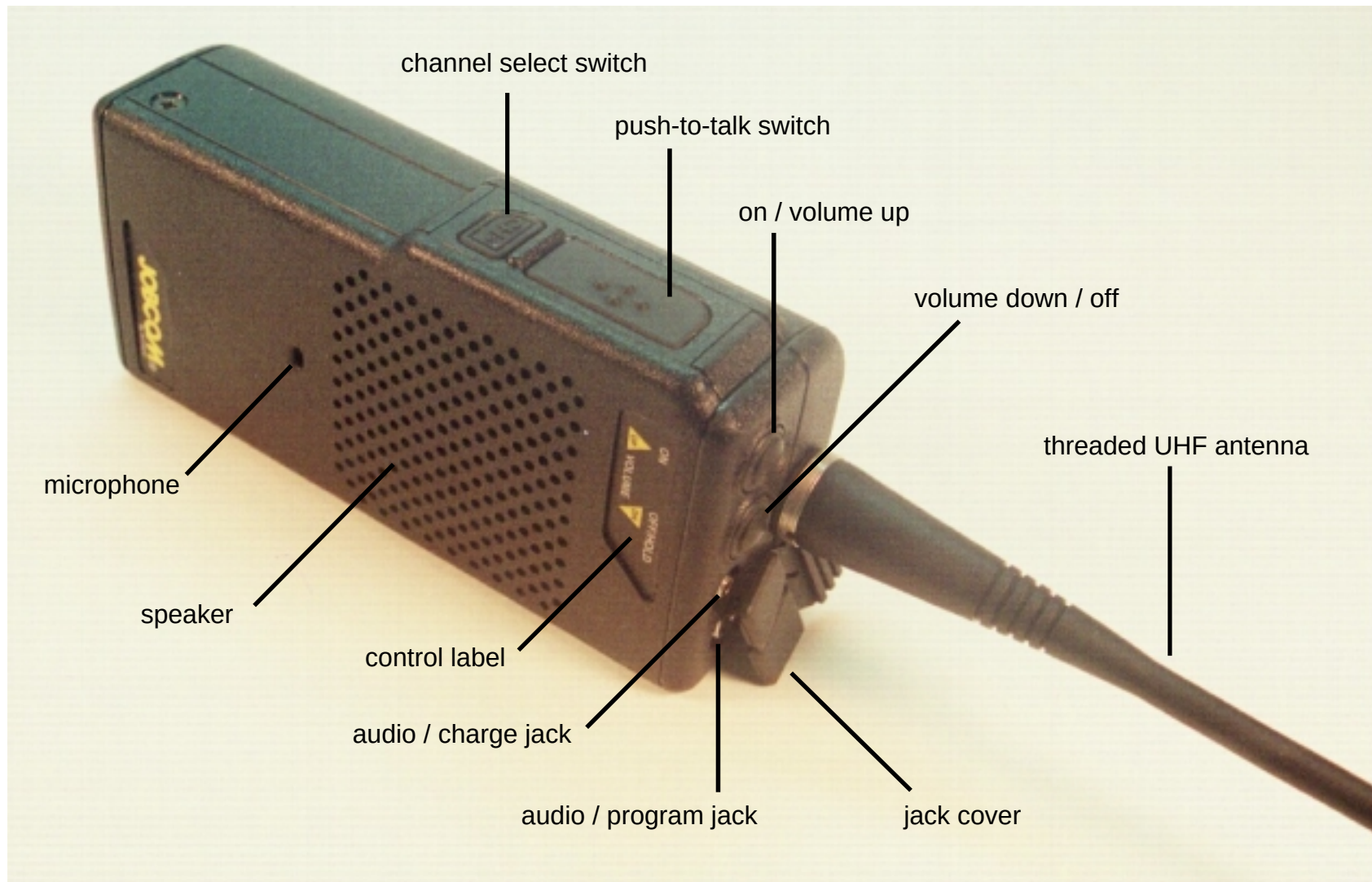
AIERIT13-450 SST-444 controls, jacks, and control label.
