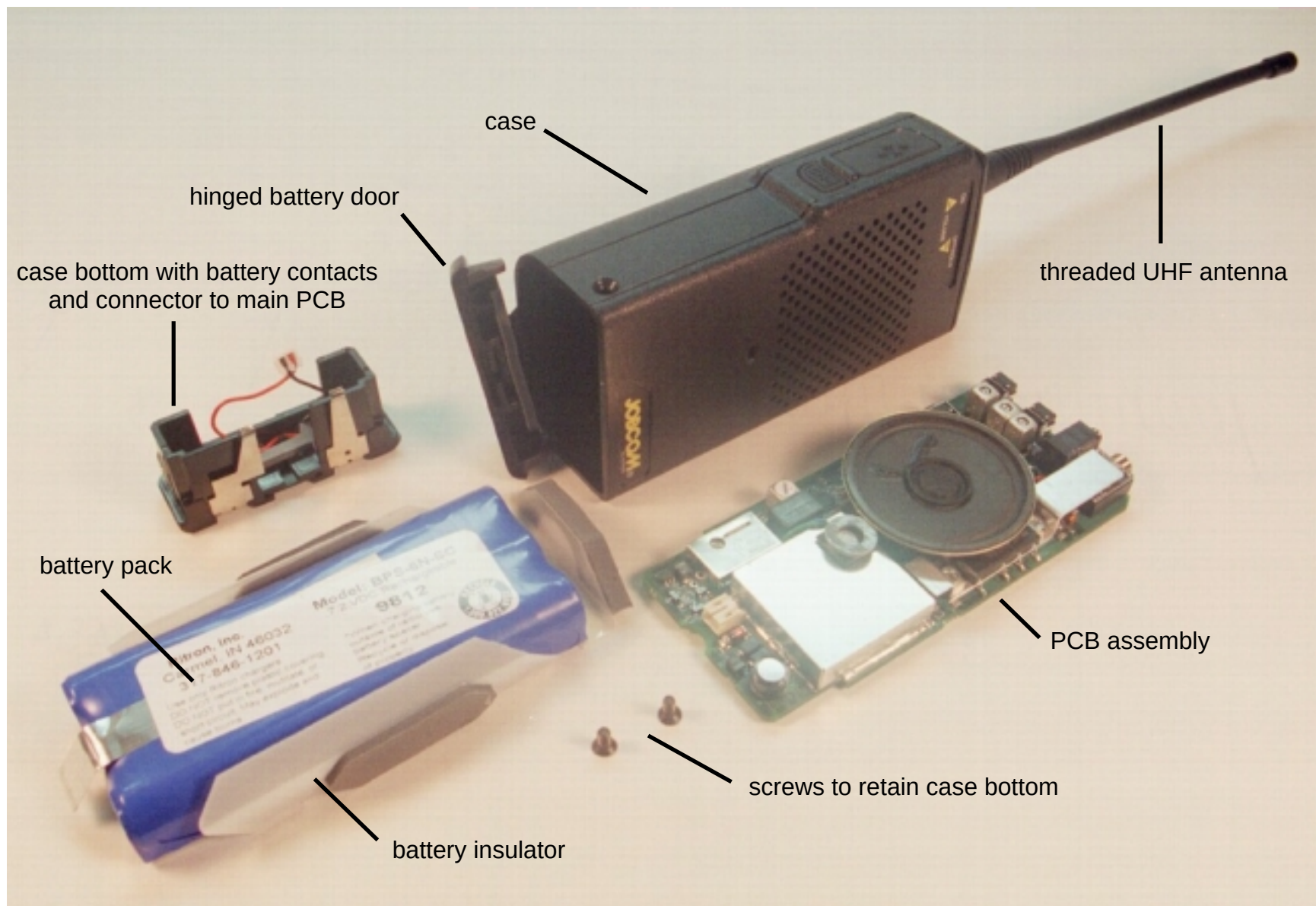
AIERIT13-450 SST-444 case assembly components.
