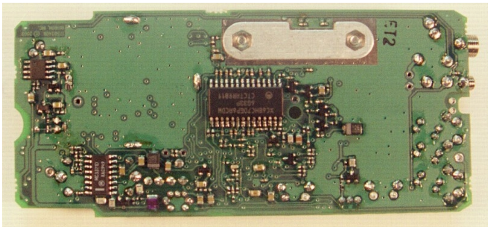
AIERIT13-450 SST-444 complete bottom side PCB assembly
