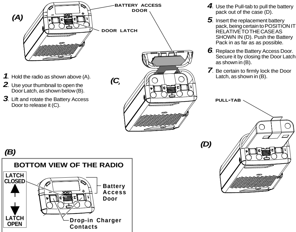
FIG-5: BATTERY ACCESS & INSTALLATION:
