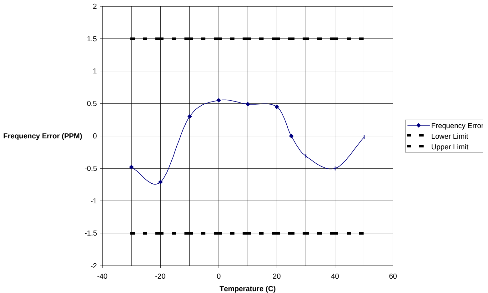
Frequency Error VS Temperature
