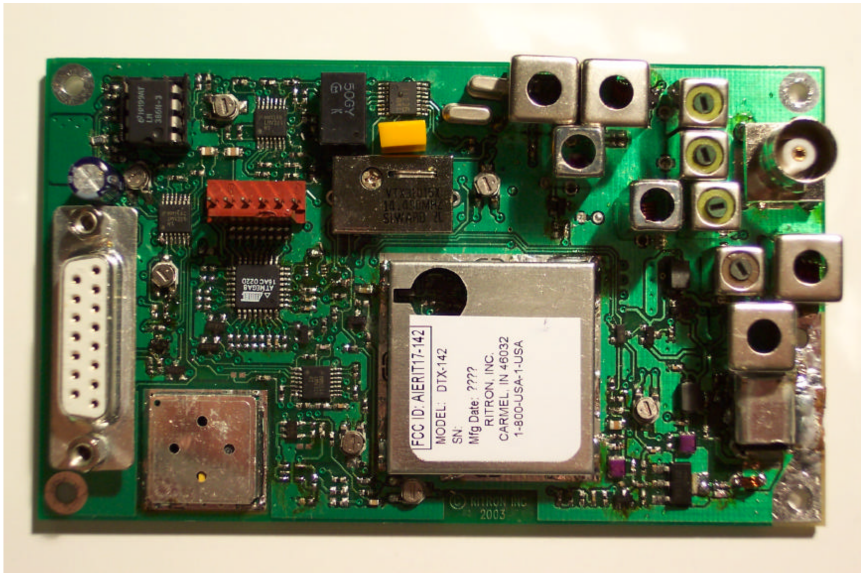
Top view of DTX-142 with shield in place.
