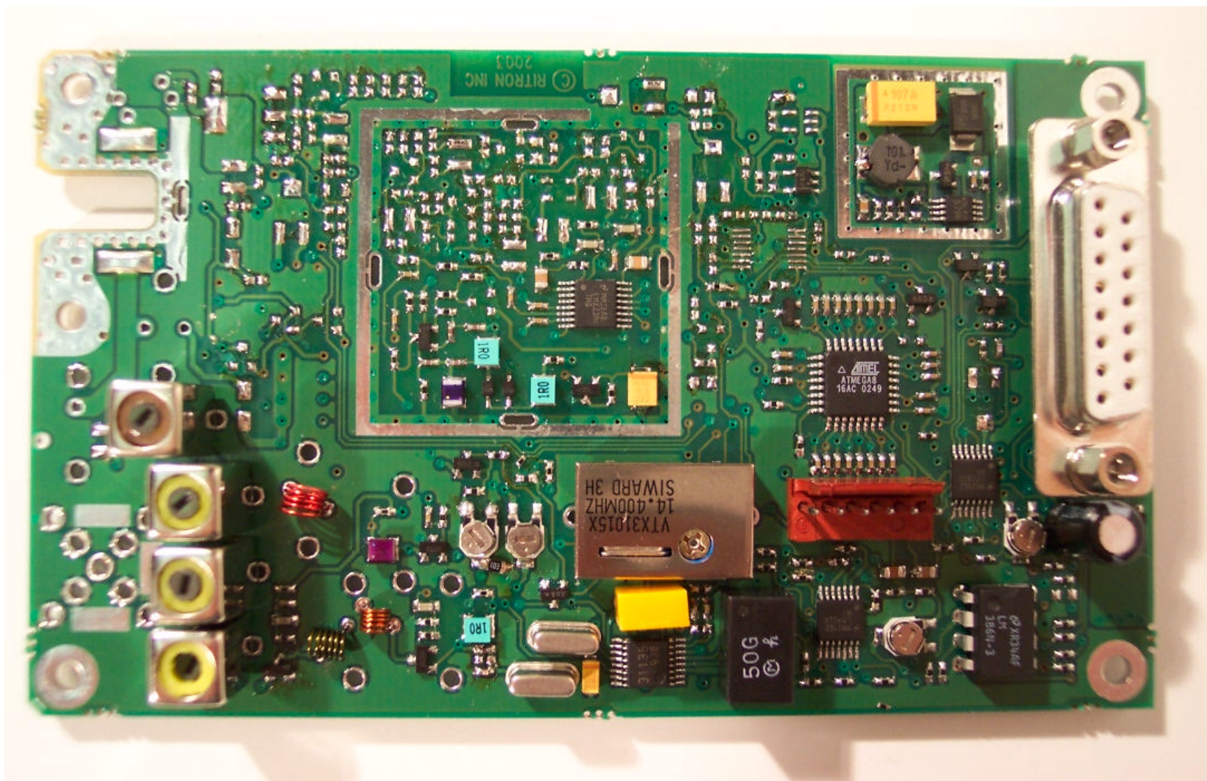
DR-142 PCB top without shields.
