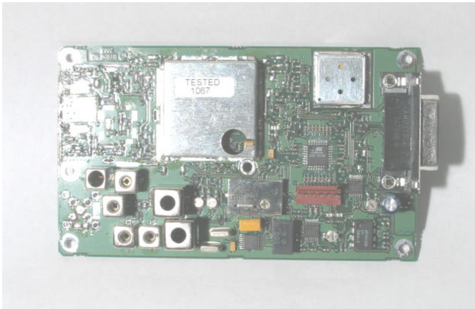
DR-442 PCB top with shield.
