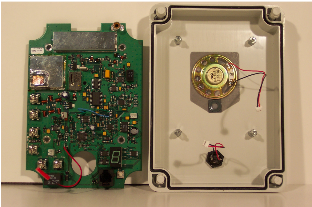
EXHIBIT: RQX-156 with printed circuit board removed from front case
