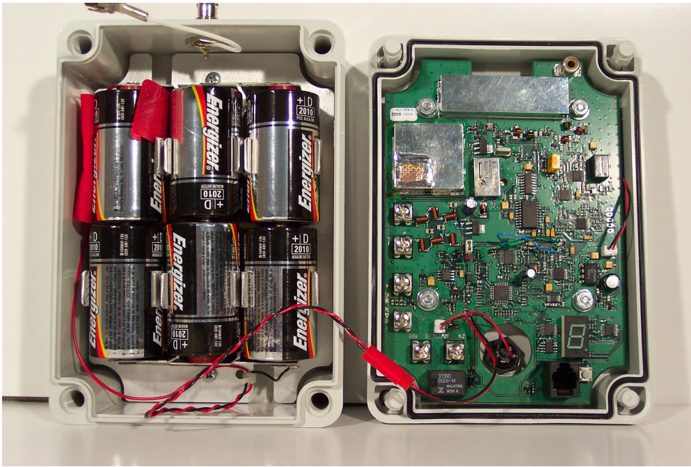
EXHIBIT: RQX-156 with case open to show printed circuit board installation
