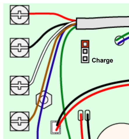
FIG-4: Charge Jumper in Charge Position
