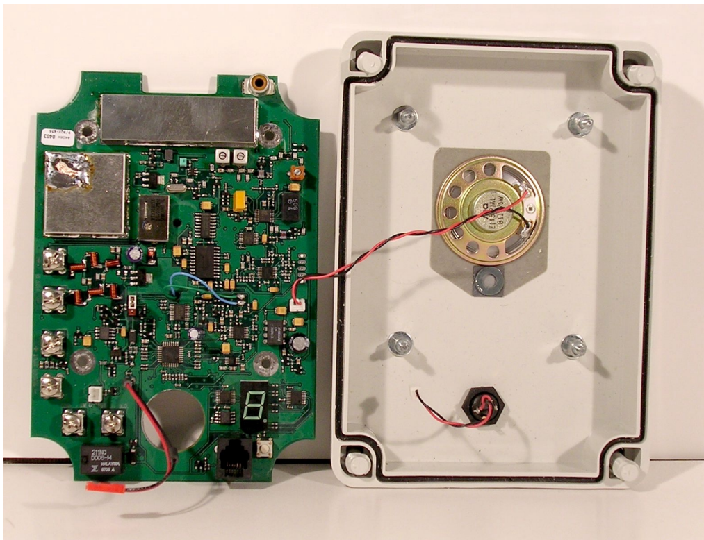
EXHIBIT: RQX-456 with printed circuit board removed from case front
