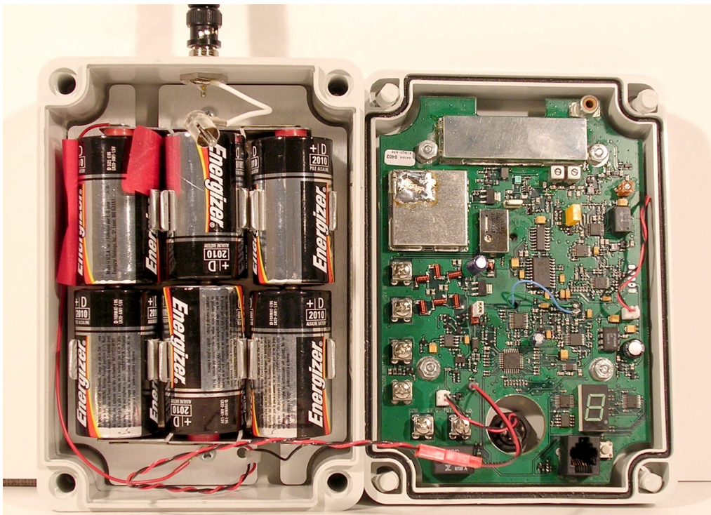
EXHIBIT: RQX-456 with case open to show printed circuit board installation
