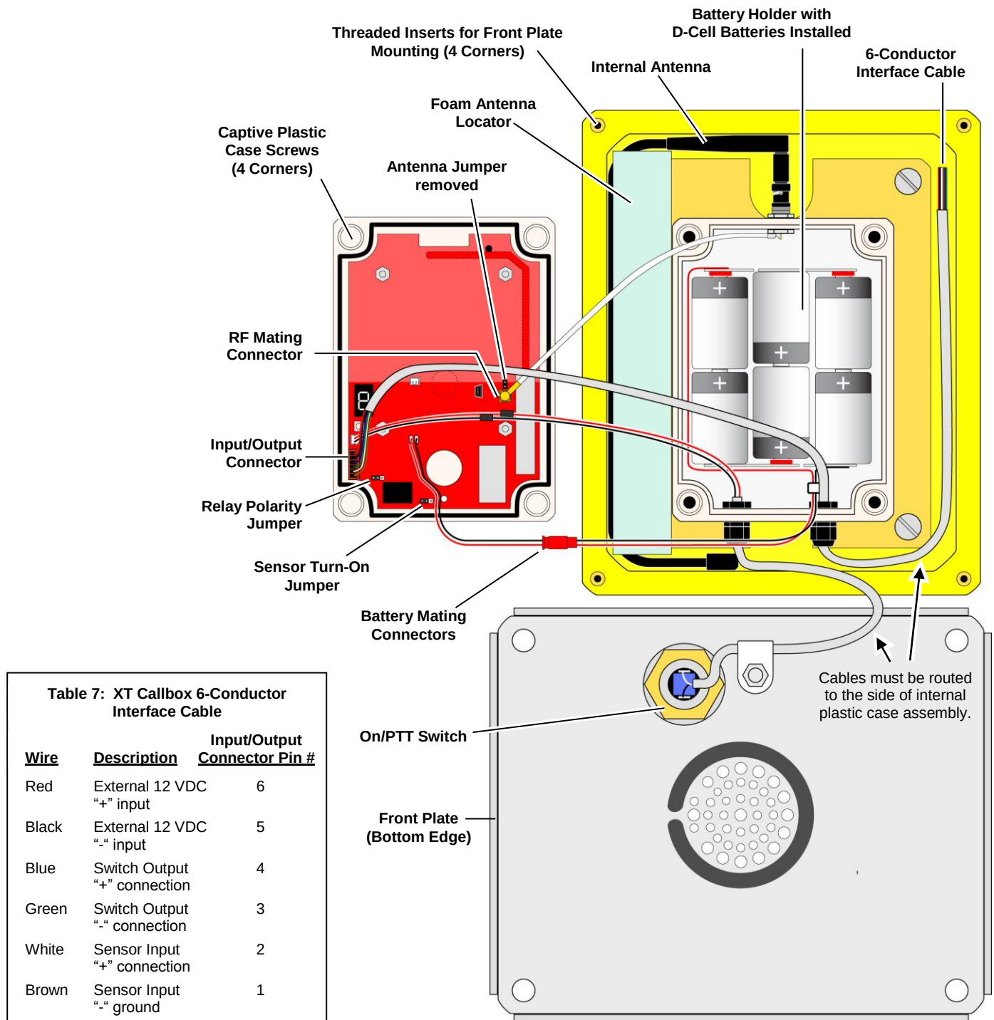
FIG: 6 XT CALLBOX ASSEMBLY.....
