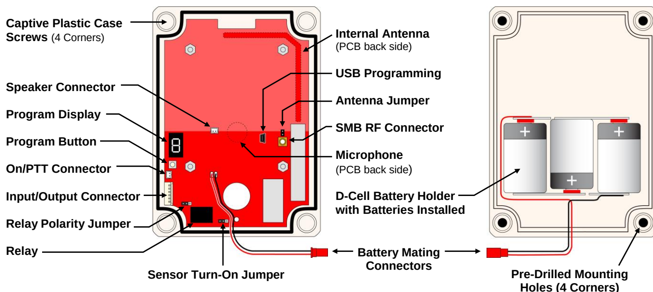
FIG-3: Callbox Assembly, Controls and Connectors
