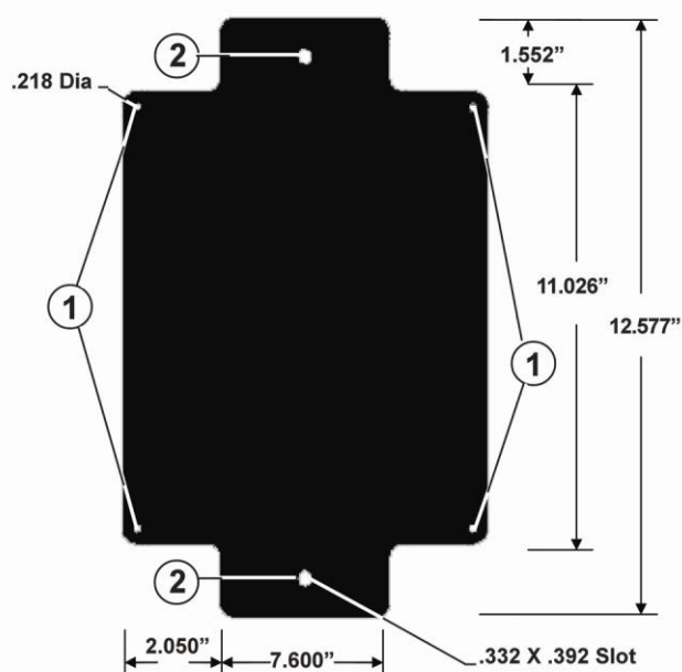
FIG-5: Optional XTMK Mounting Bracket XT Callbox
