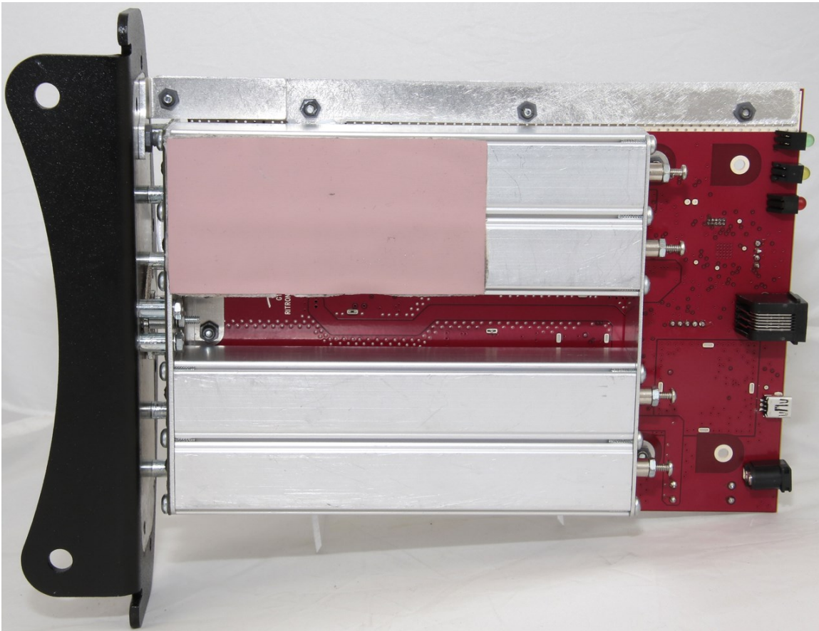
RLR-465 bottom view with duplexer and heatsink
