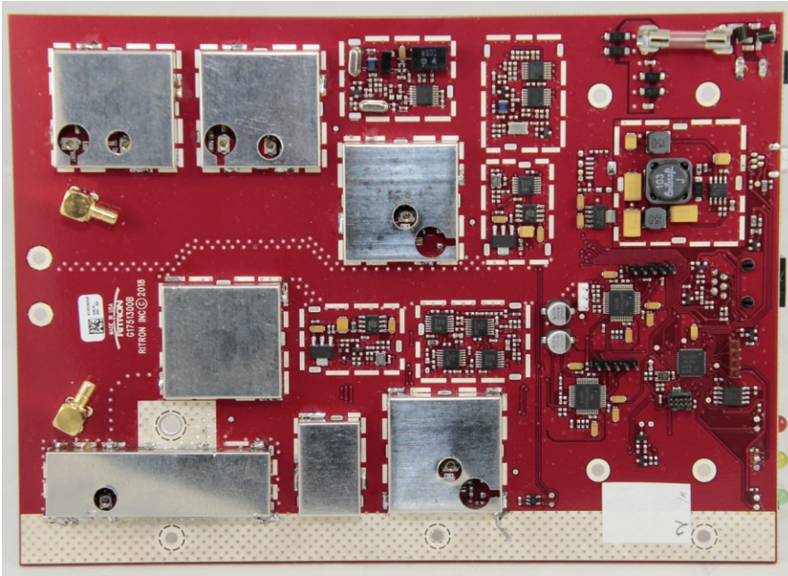
RLR-465 top view with shields
