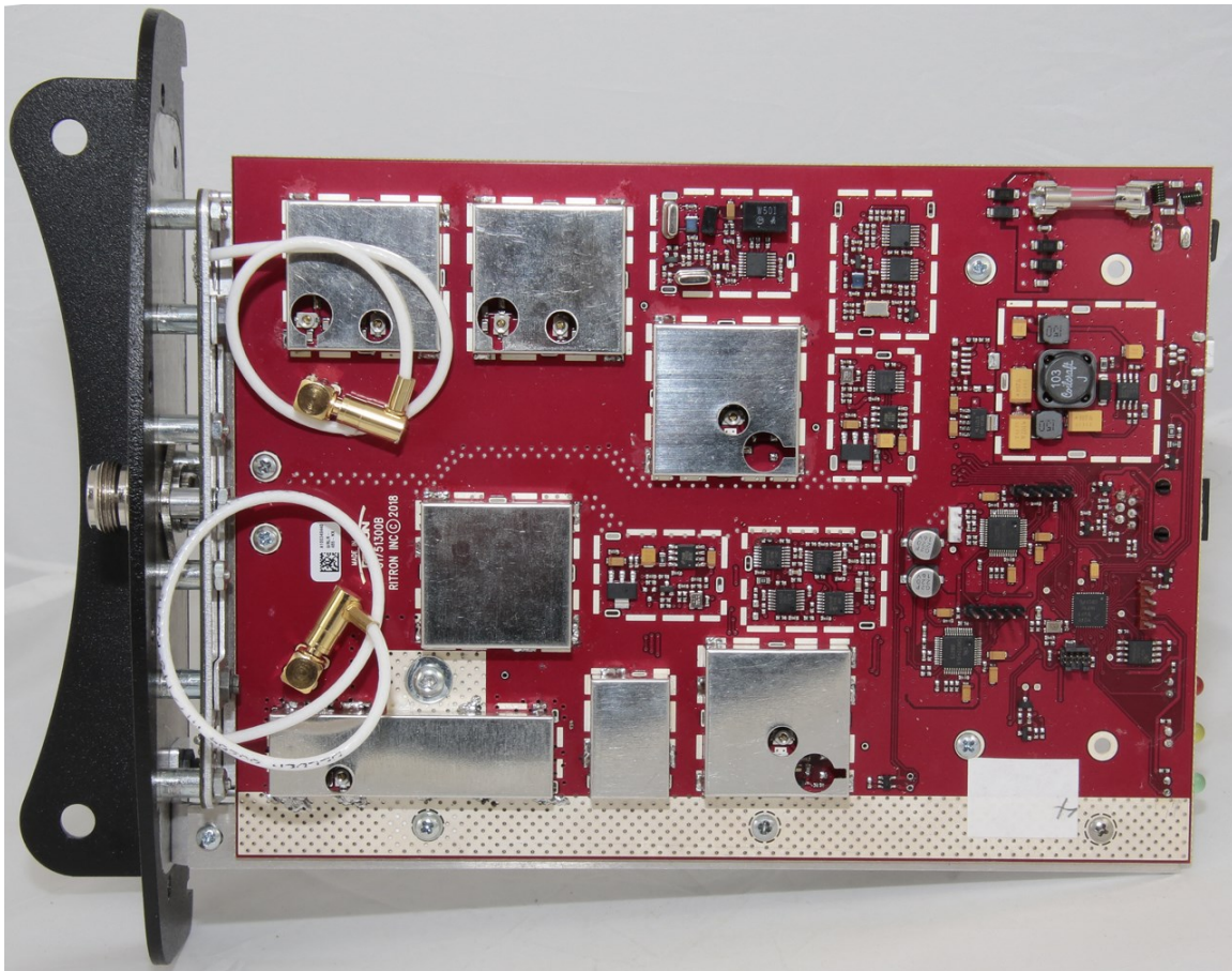
RLR-465 top view with heat sink and duplexer below PCB
