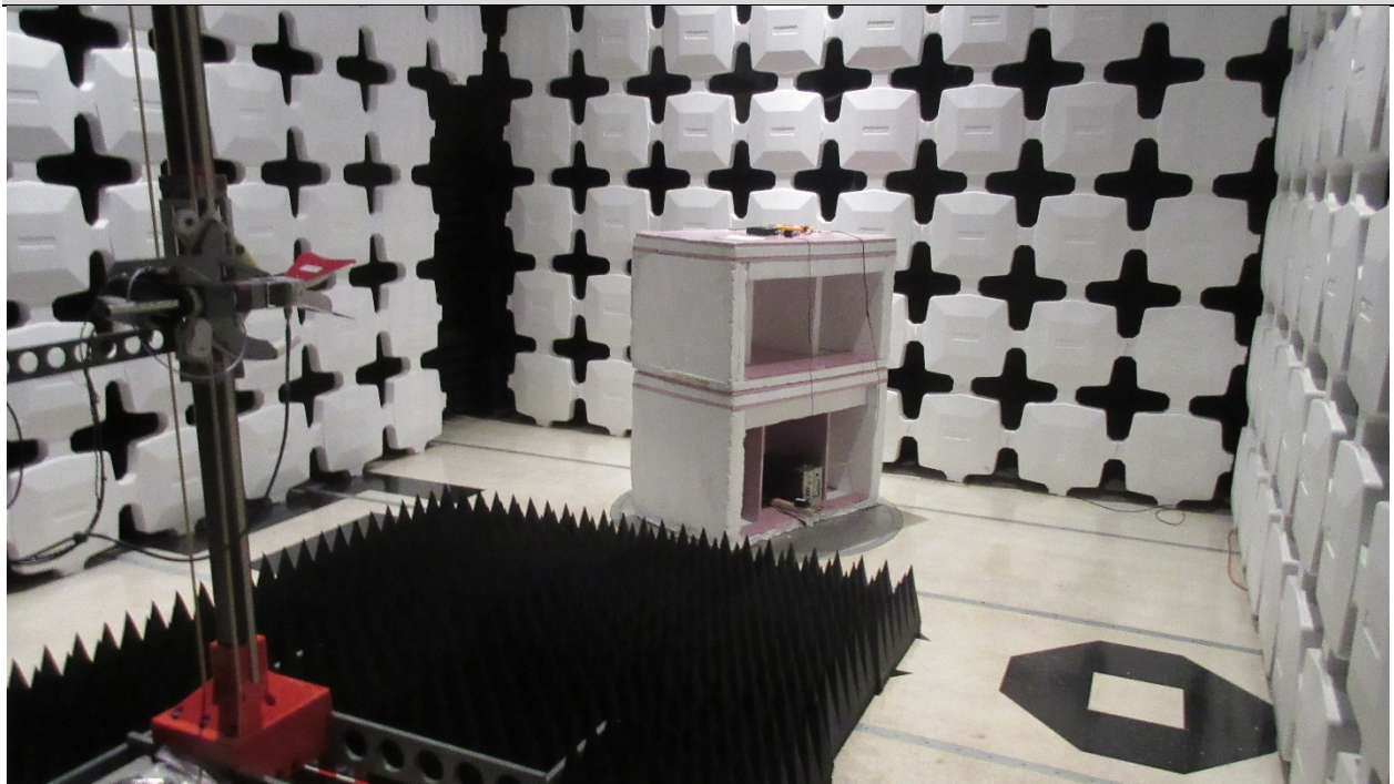
Radiated, Below 1 GHz #2
