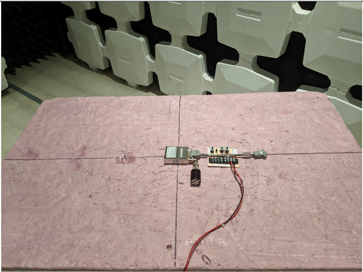
Radiated, Table Setup
