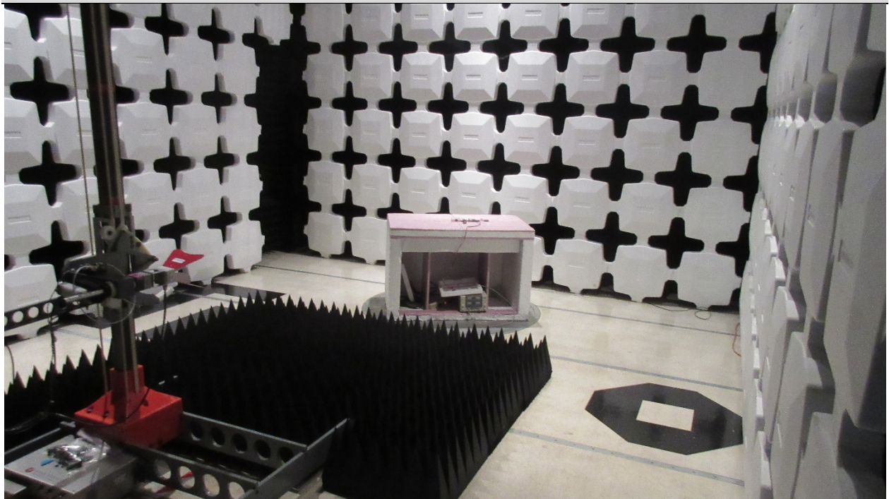
Radiated, Above 1 GHz
