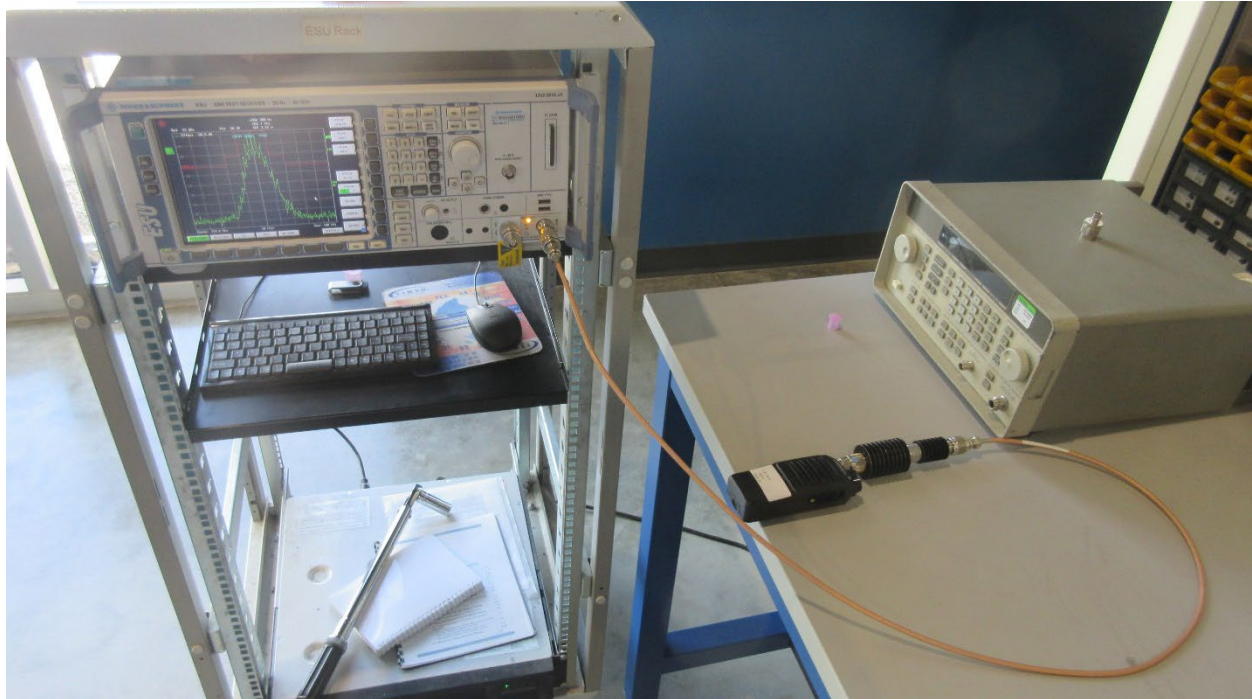
Conducted Test Setup
