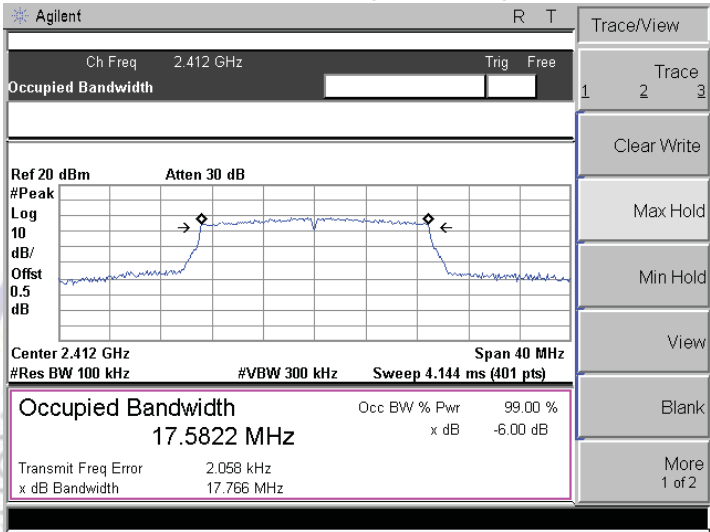
Channel 01 (2412MHz)
