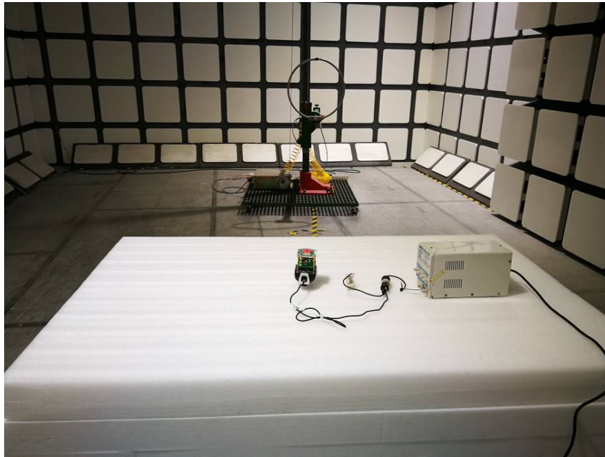
Radiated Emissions View (9k-30MHz)
