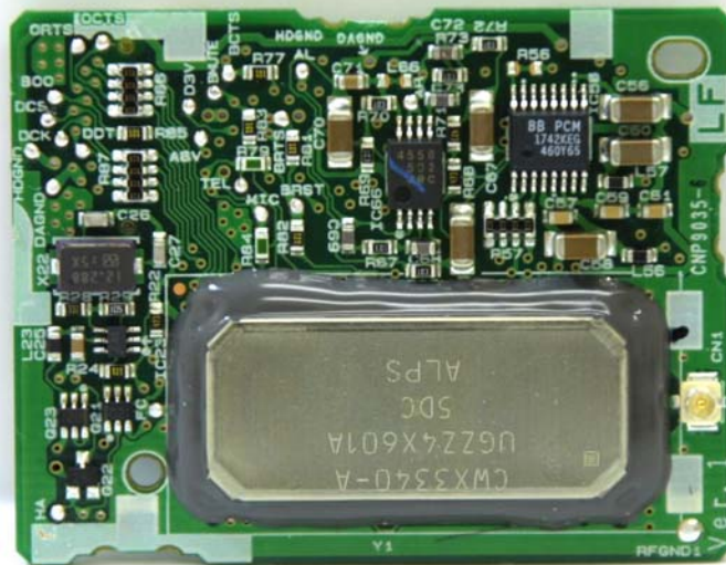
Front Side without shielding (Bluetooth Unit)
