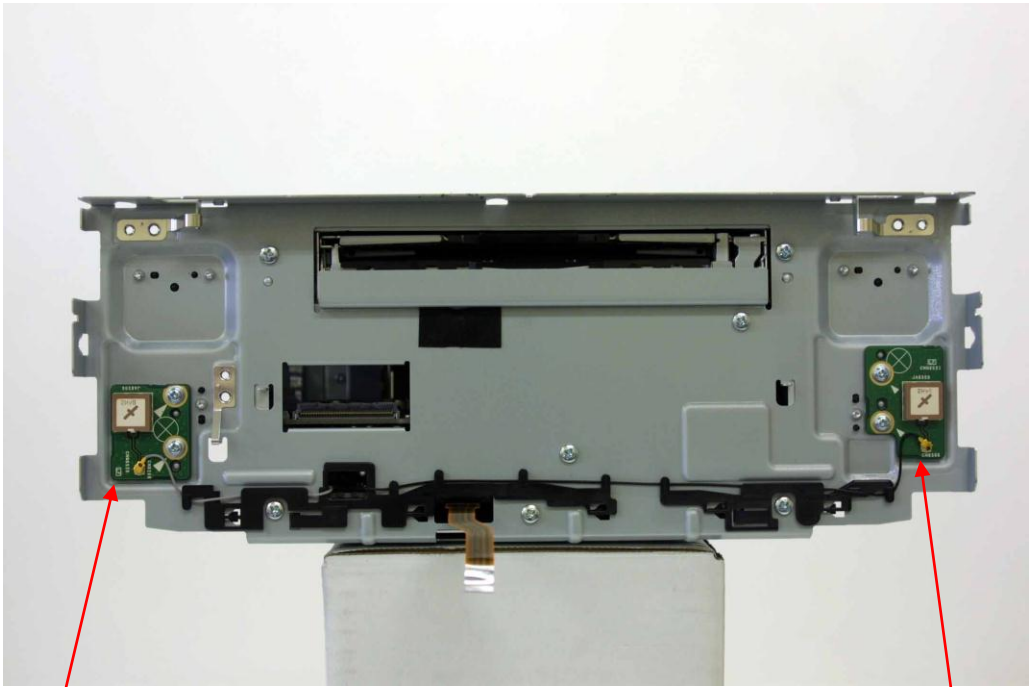
WLAN Antenna
