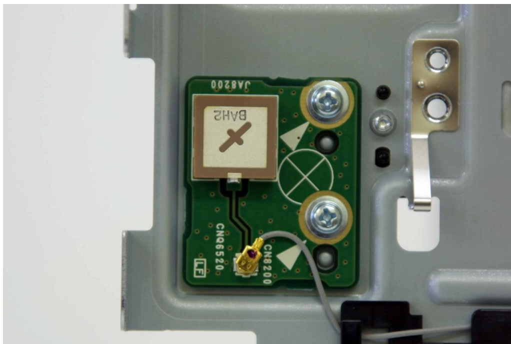
WLAN Antenna
