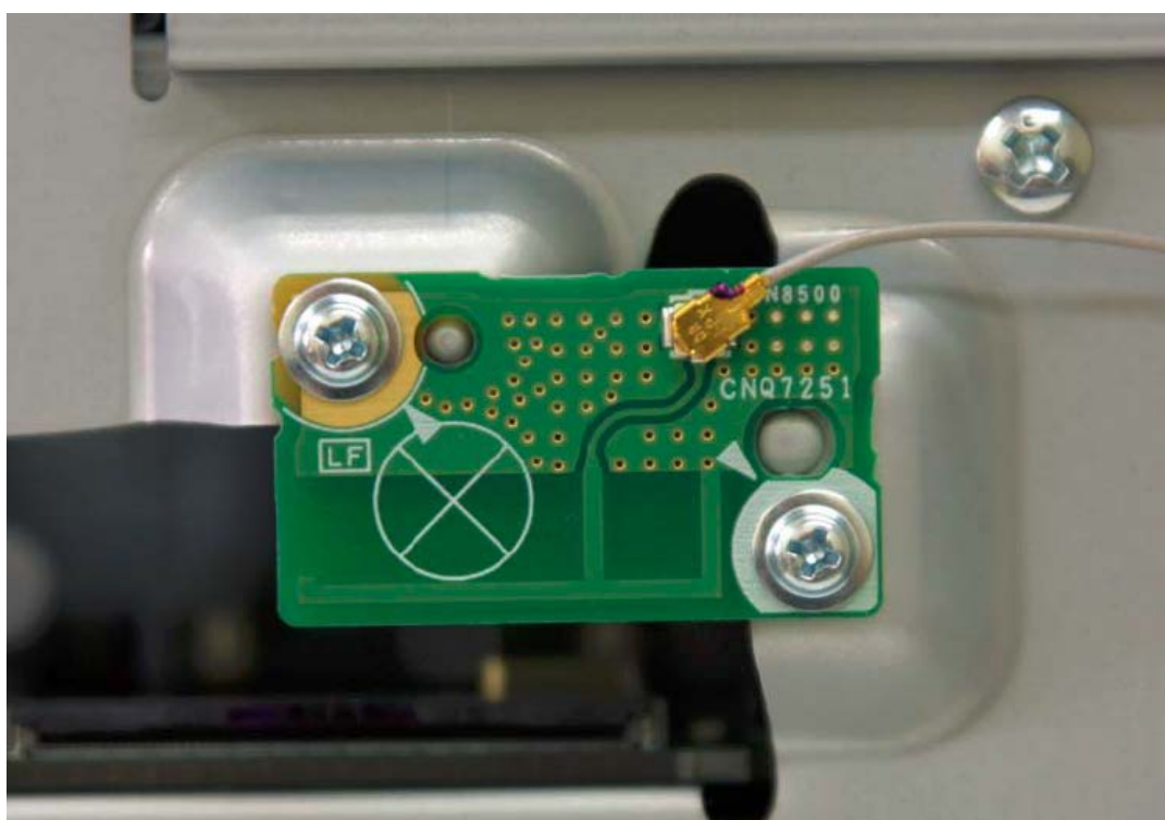
Bluetooth antenna
