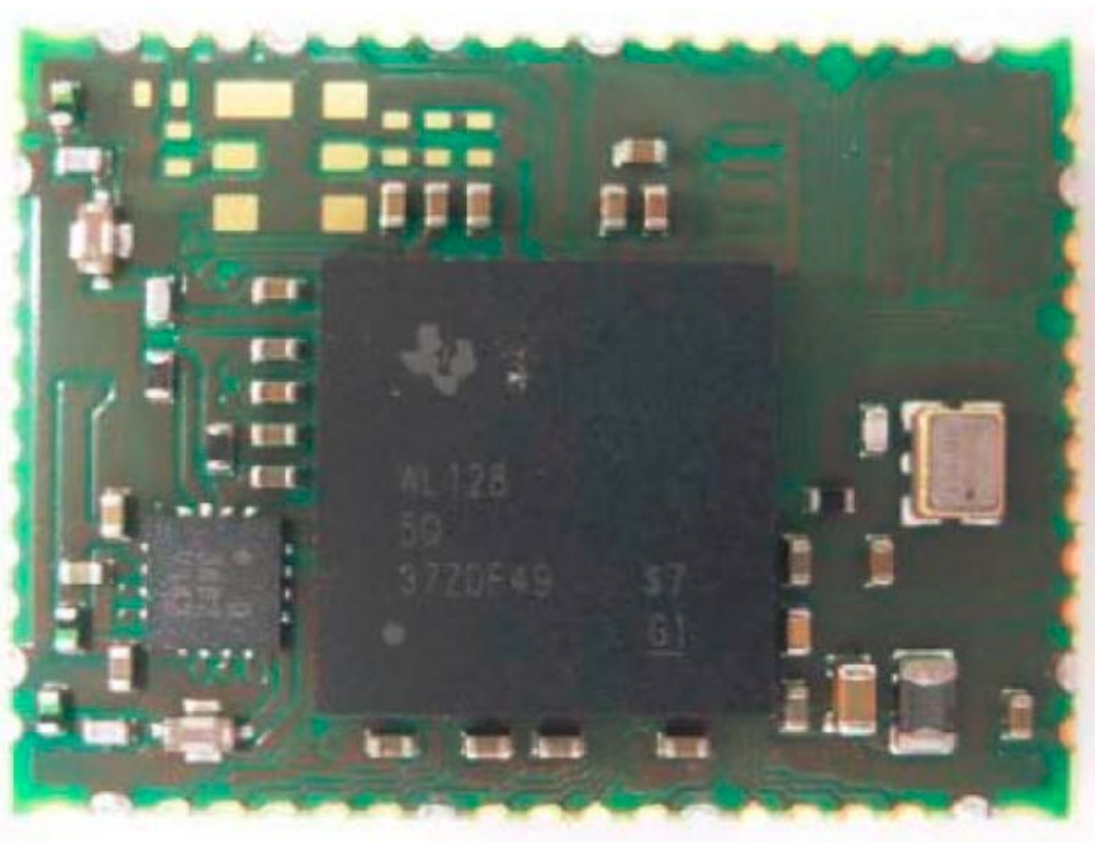
RF Module without Shield
