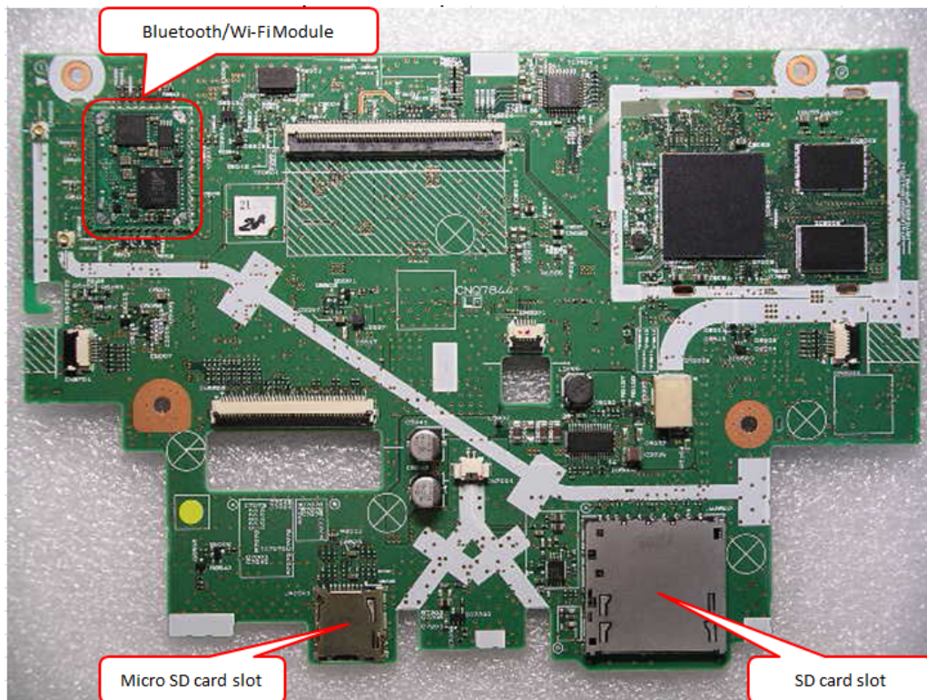
Electronic Board surface side (without shield)
