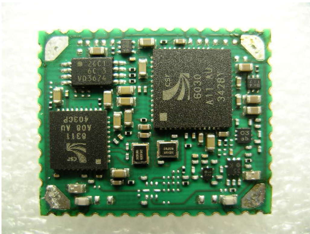
Module surface side (without shield)
