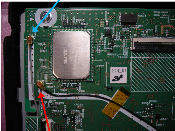
Wi-Fi Antenna Connector
