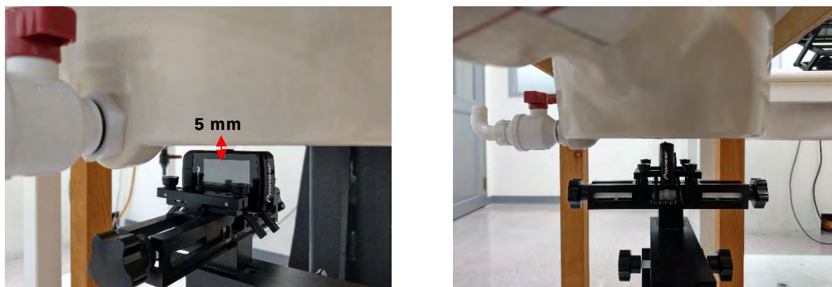
Fig.9 EUT Left side to flat phantom
