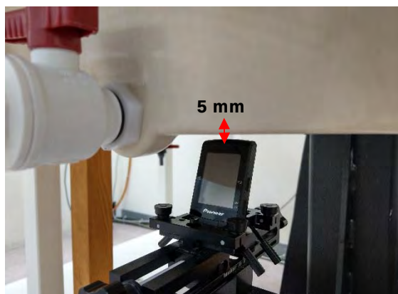
Fig.6 EUT Top Tilt side to flat phantom
