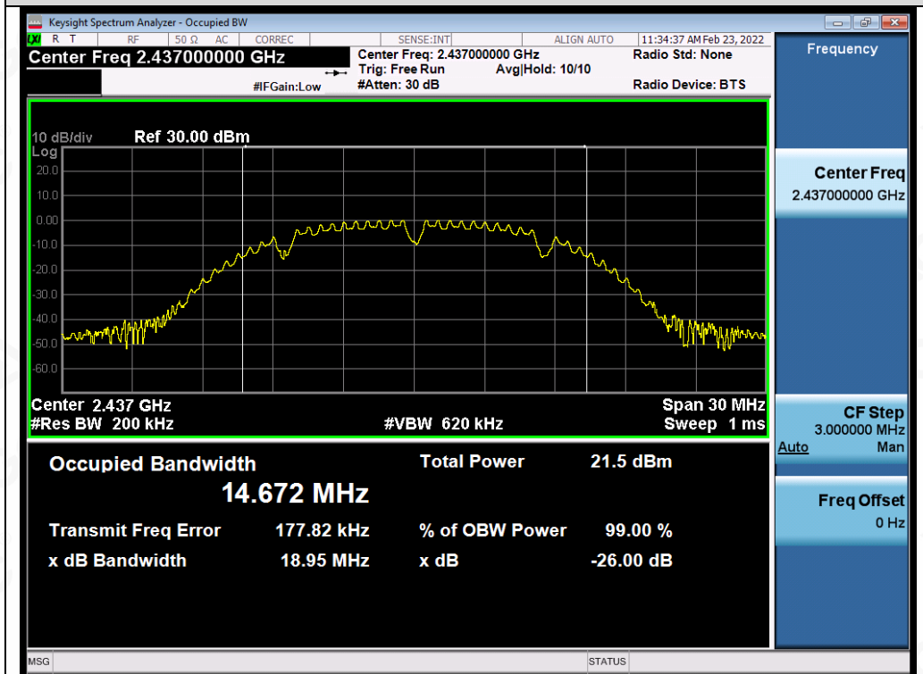
Test_Graph_802.11n20_ANT1_2437_MCS0_OBW
