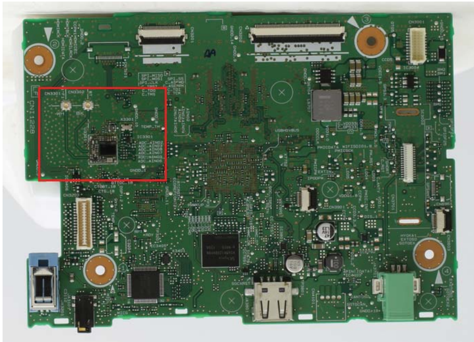
PCB side A
