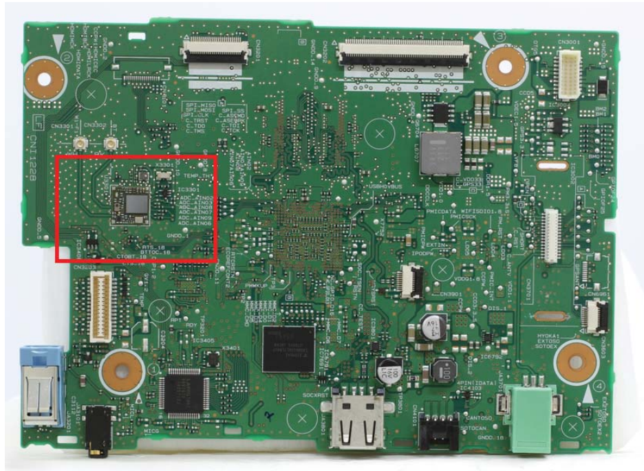
PCB side A
