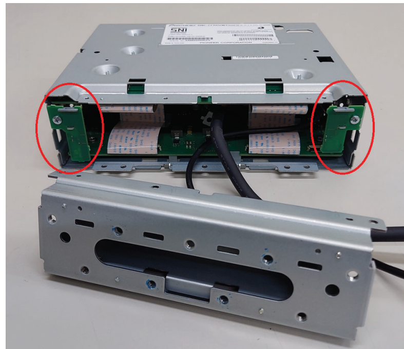
Bluetooth Antenna (2.4GHz)
