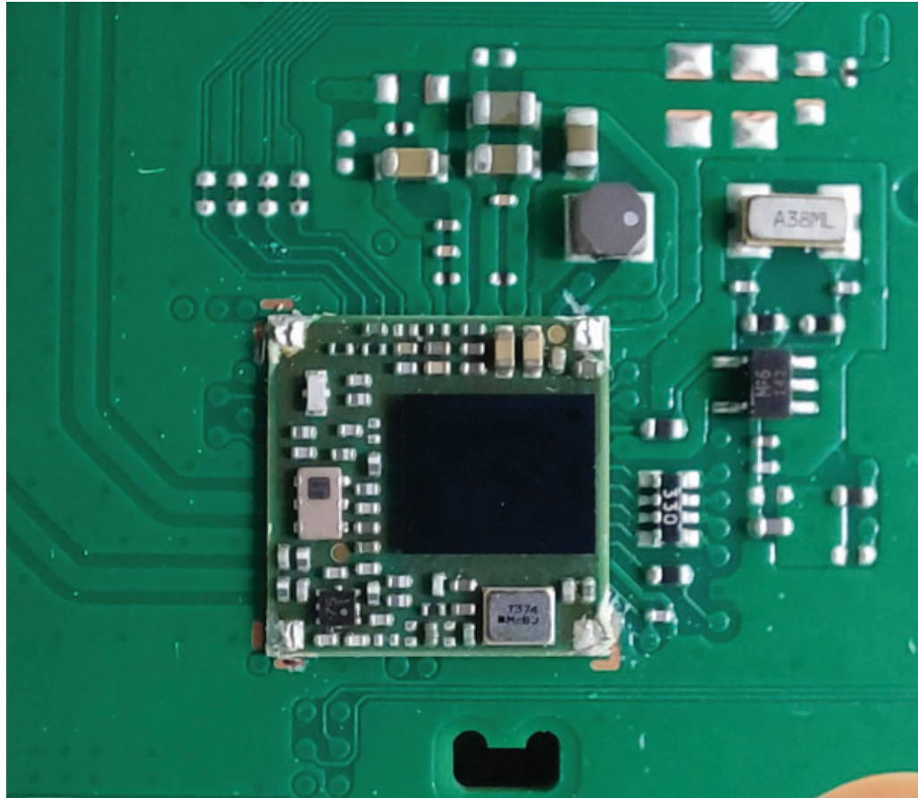
RF Module (shield case removed)
