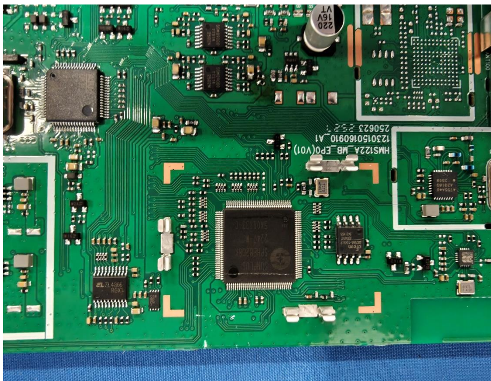
Photo 8: Internal View for PCB A
