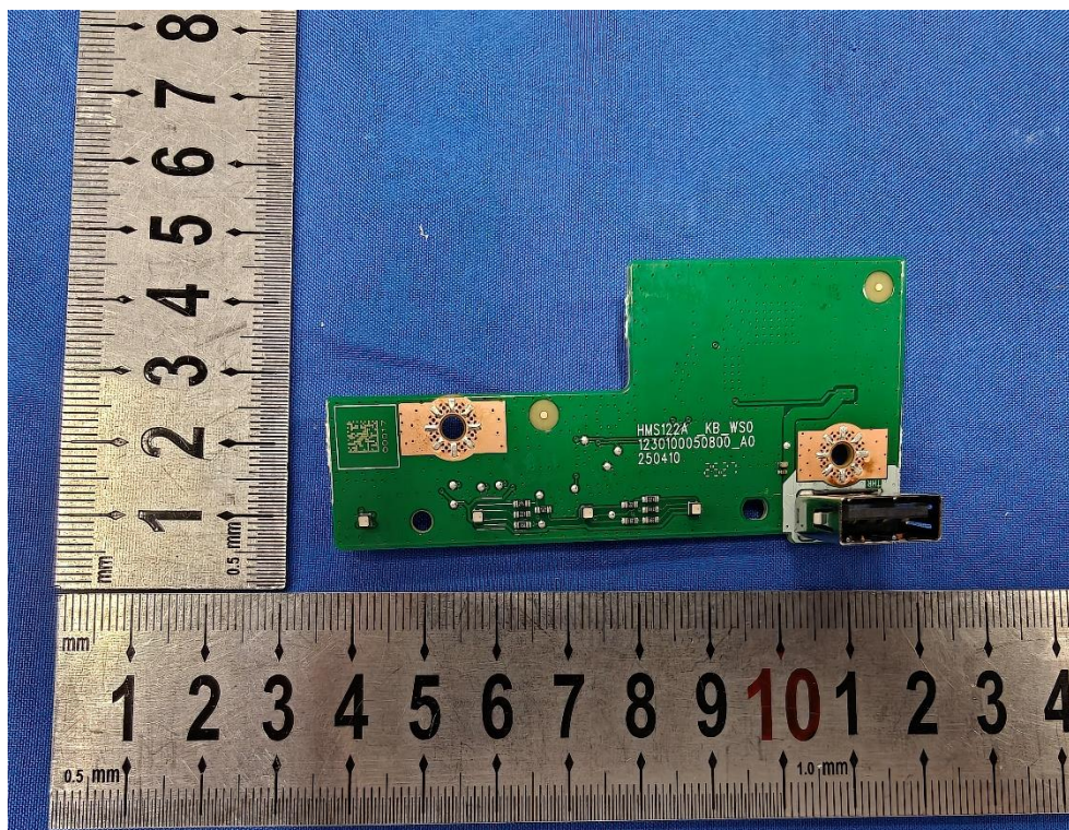
Photo 5: Internal View for PCB B
