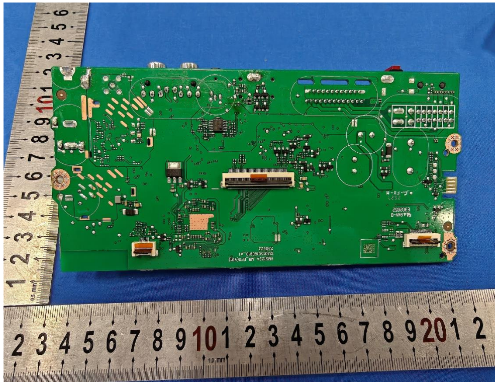
Photo 3: Internal View for PCB A
