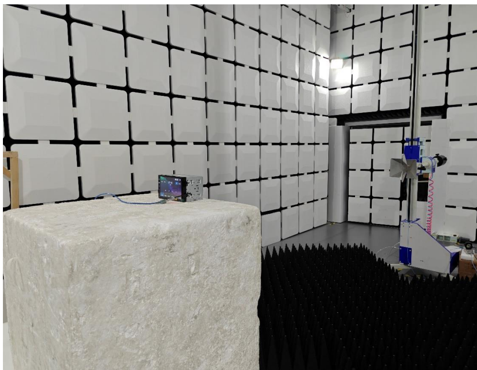
Description: RF Radiated Emission Test Setup for 1GHz ~ 18GHz
