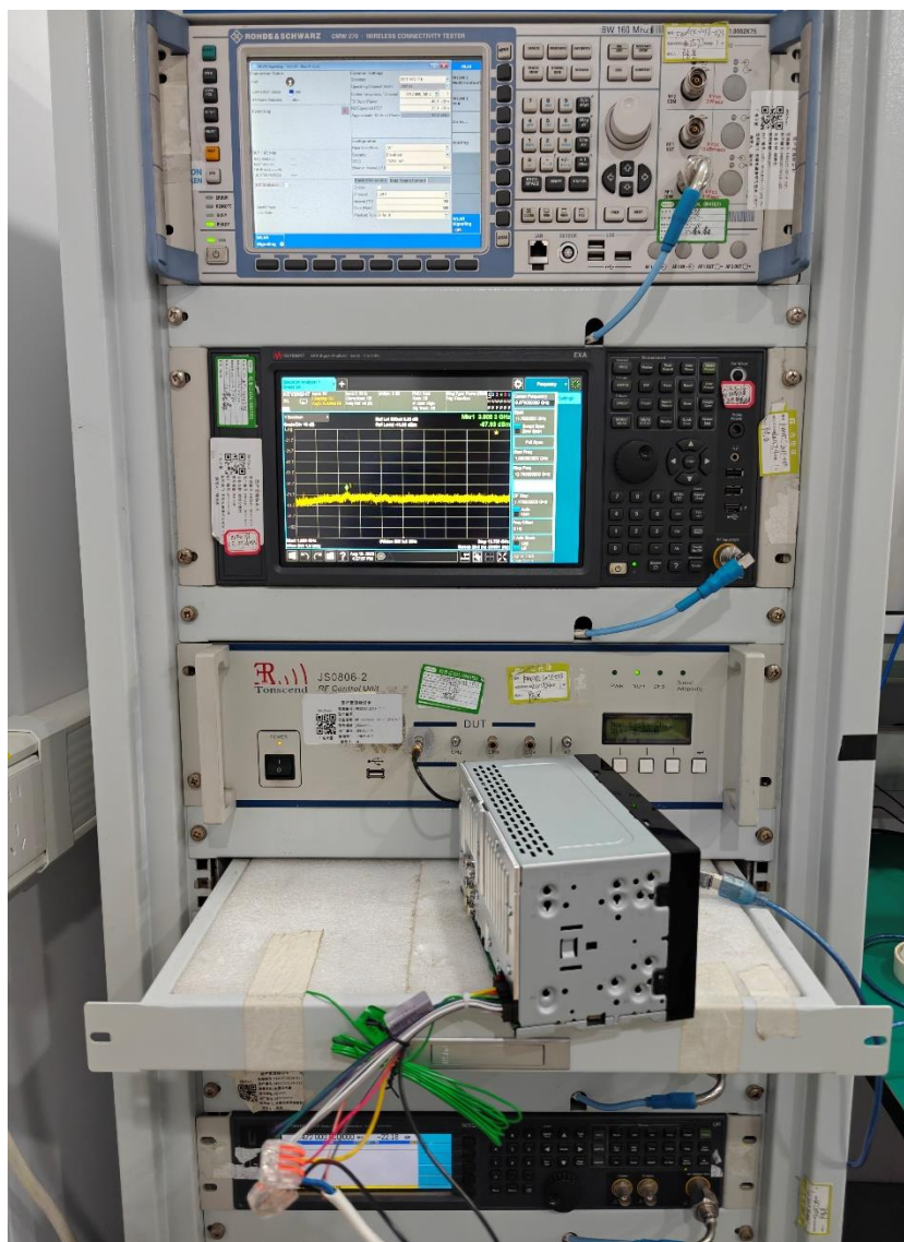
Description: RF Conducted Test Setup Photo
