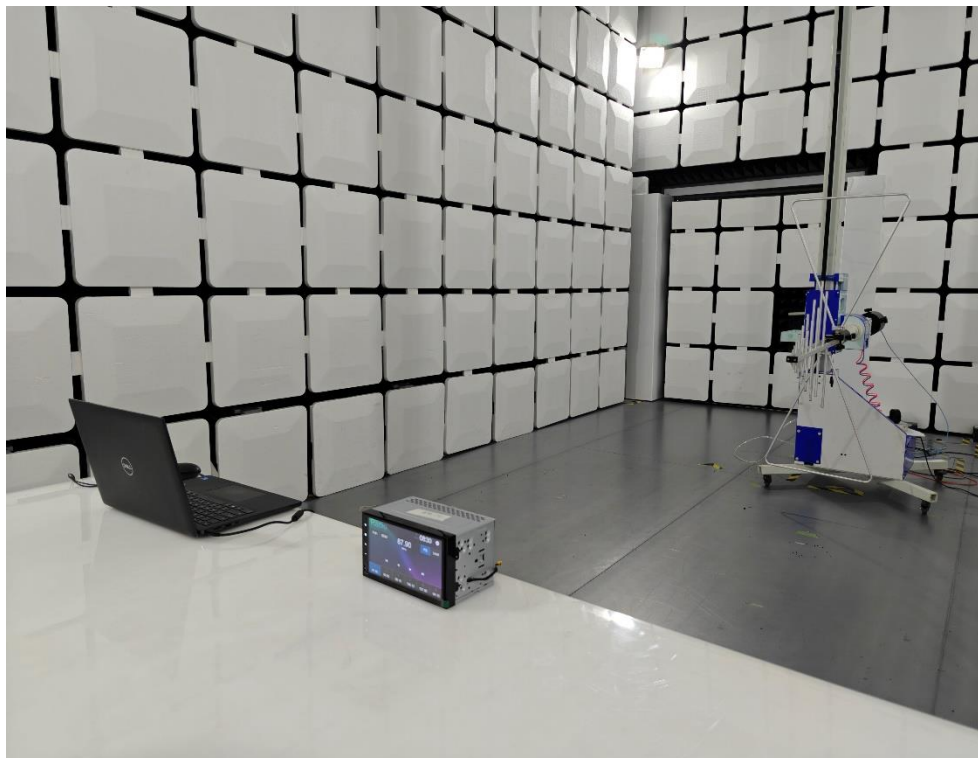
Description: RF Radiated Emission Test Setup for 30MHz ~ 1GHz
