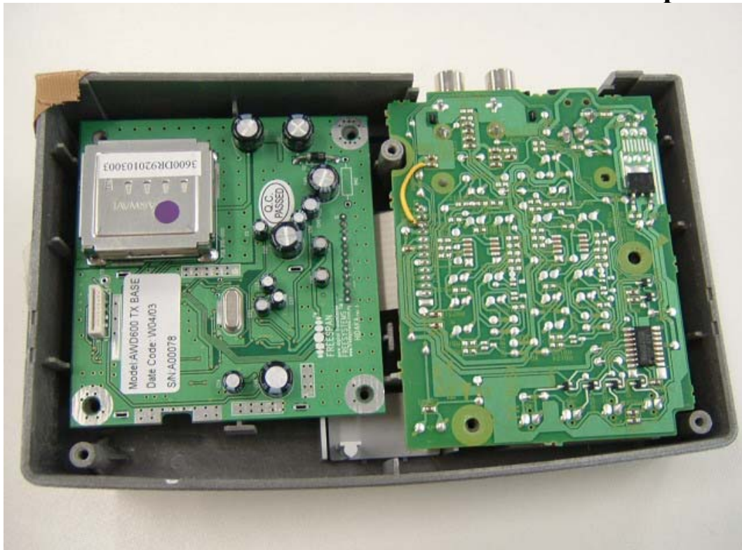
Front side with shield
