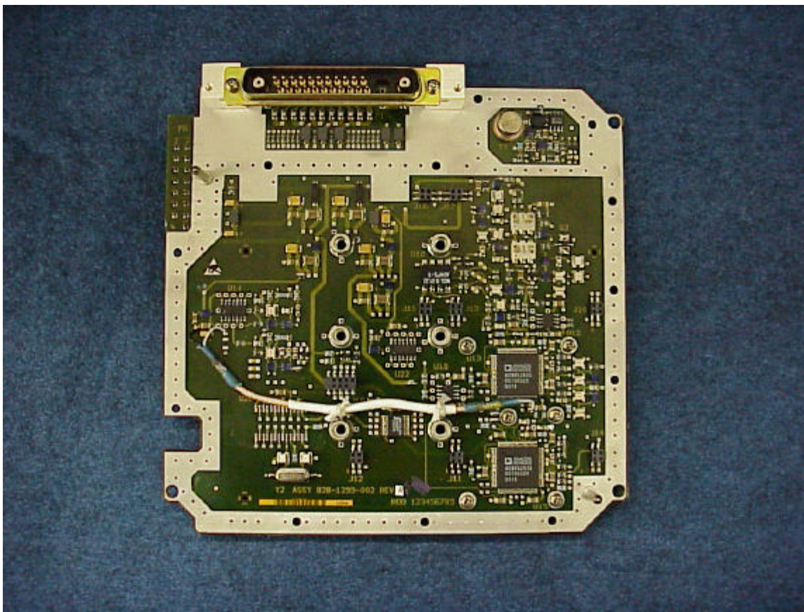
Figure 8-6. Source Digital Top
