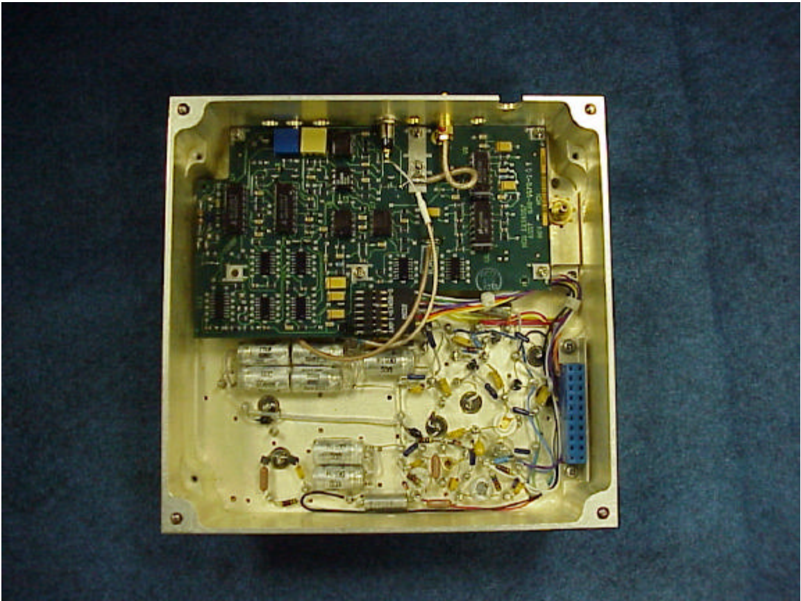
Figure 8-3. Driver Rear Internal
