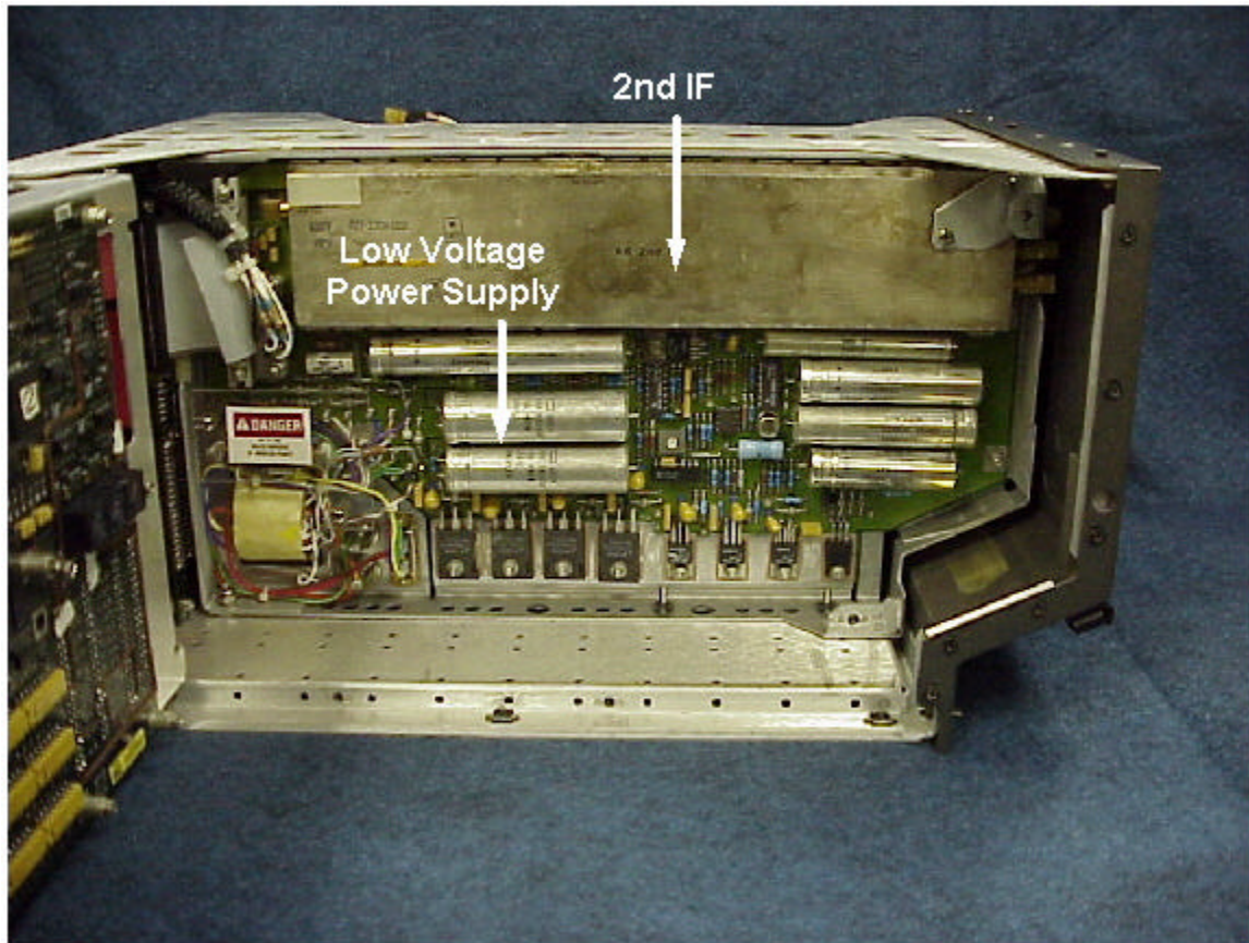
Figure 8-1. Chassis Left Open
