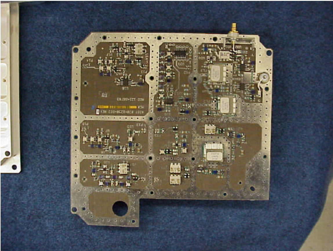
Figure 8-4. Source RF Top
