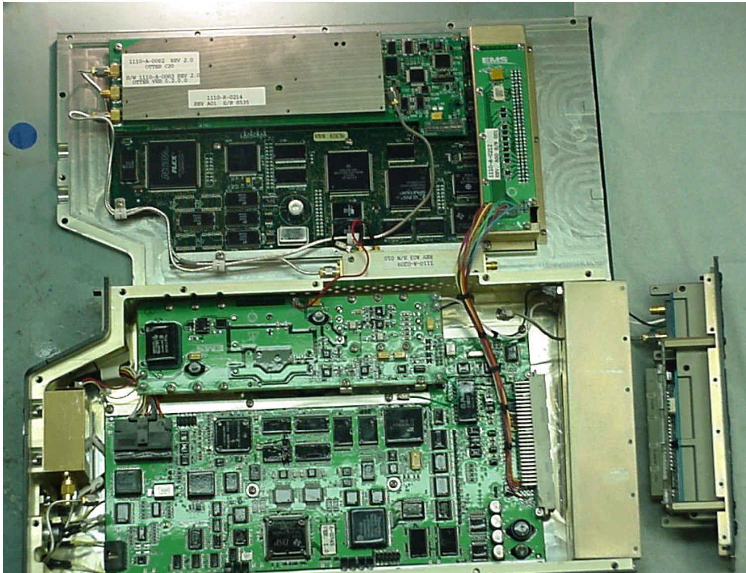
Internal View, All Assemblies
