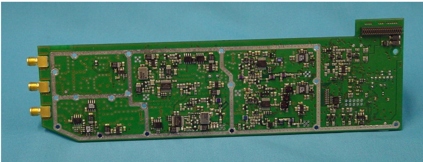
Channel Card RF Daughter board – Bottom View
