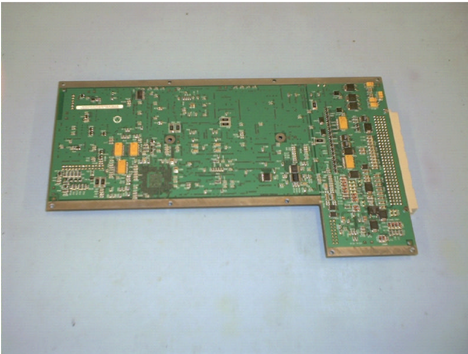
Data Processor – Bottom View
