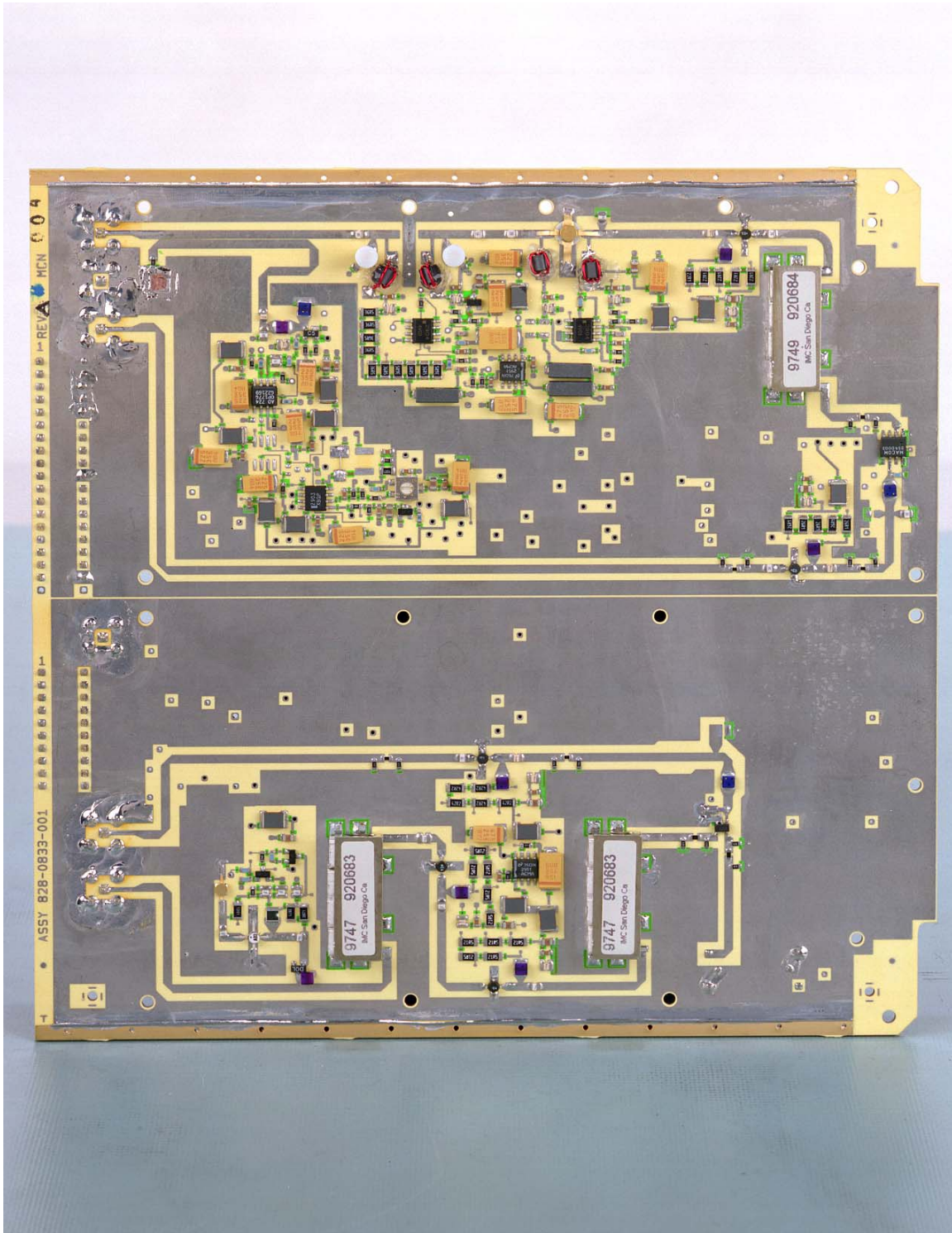
Figure 8-5. Up/Down Converter Card Assembly (Top View)
