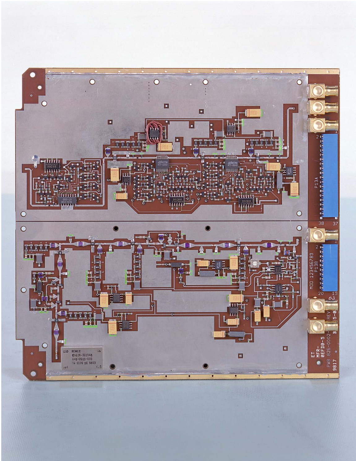
Figure 8-6. Up/Down Converter Card Assembly (Bottom View)
