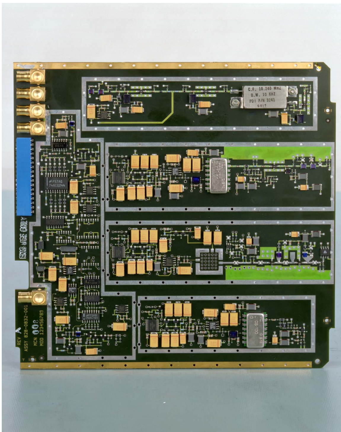
Figure 8-4. V. C. O. Card Assembly
