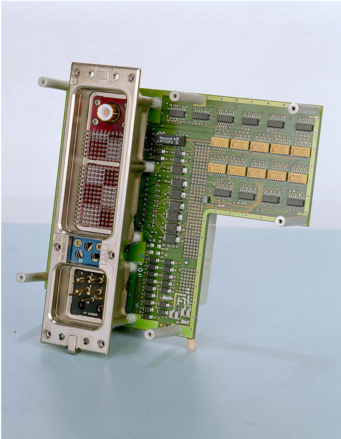
Figure 8-7. Rear Interconnect Card Assembly
