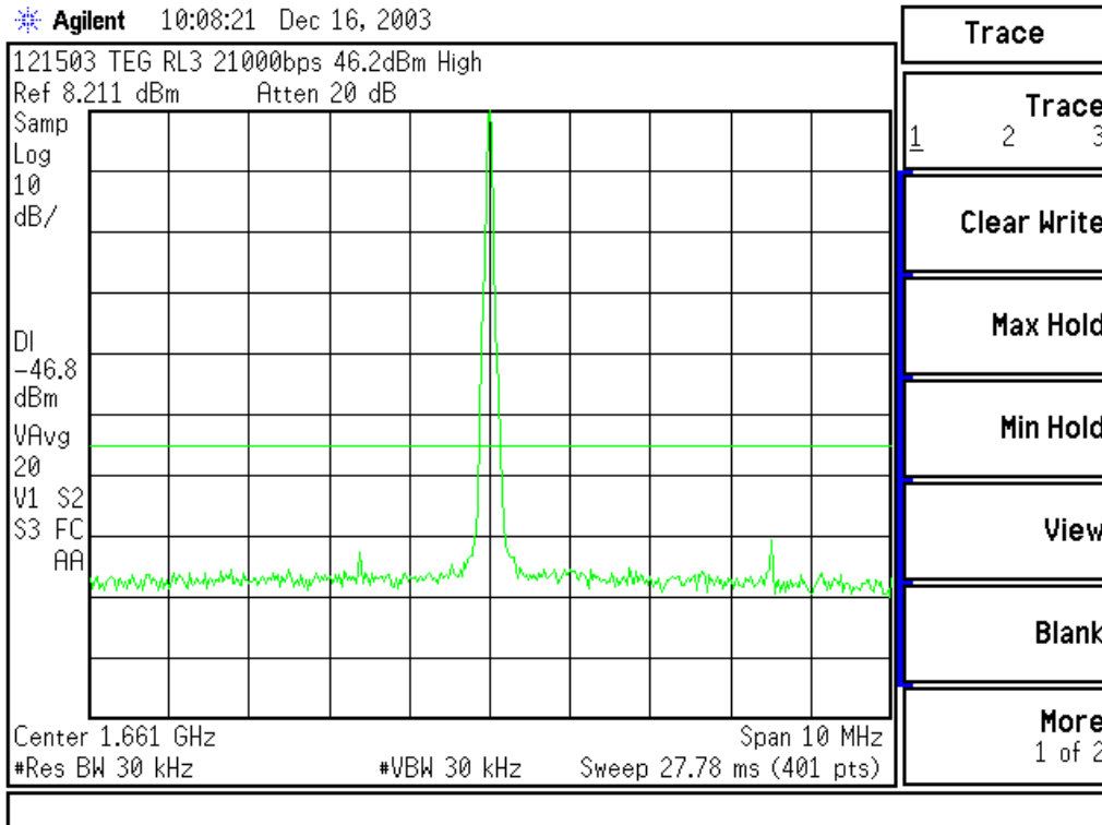
Figure 9.6.5.51. Spurious 21000 bps High Band 10 MHz Span
