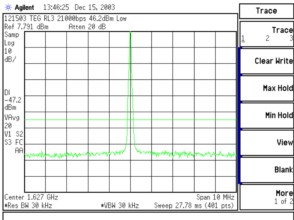
Figure 9.6.5.43. Spurious 21000 bps Low Band 10 MHz Span
