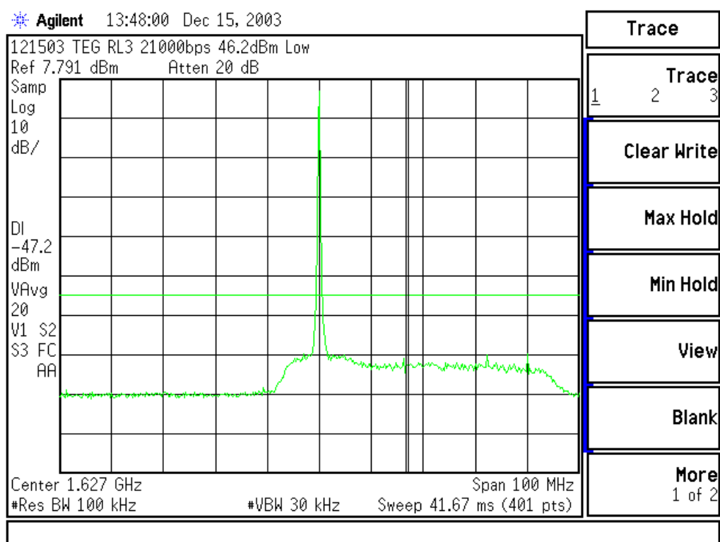
Figure 9.6.5.44. Spurious 21000 bps Low Band 100 MHz Span
