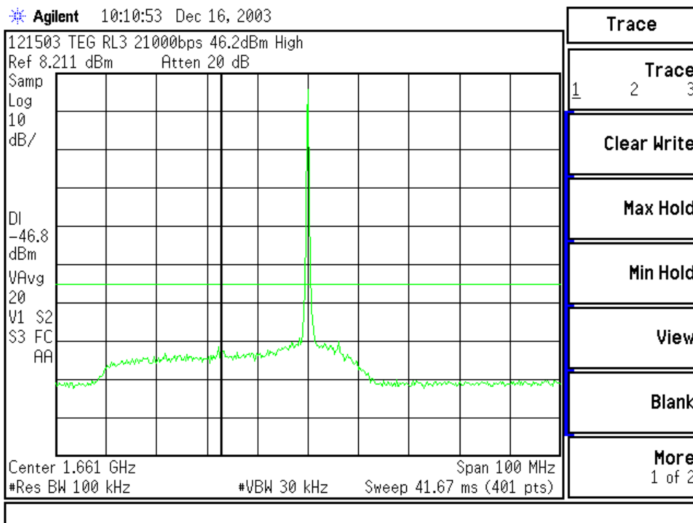
Figure 9.6.5.52. Spurious 21000 bps High Band 100 MHz Span
