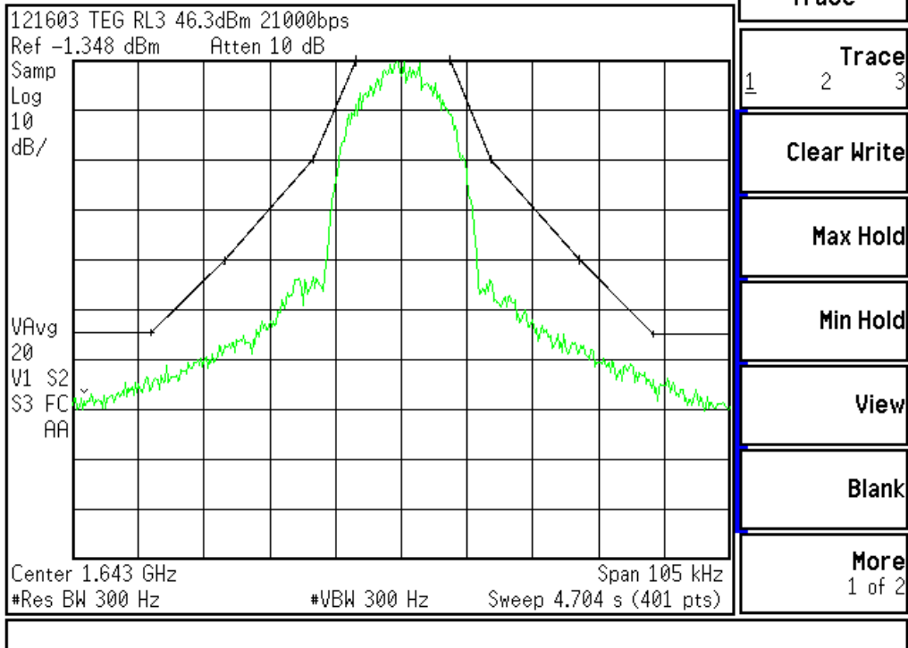
Figure 9.6.7.7. Frequency Spectrum 21000 bps 105 kHz Span
