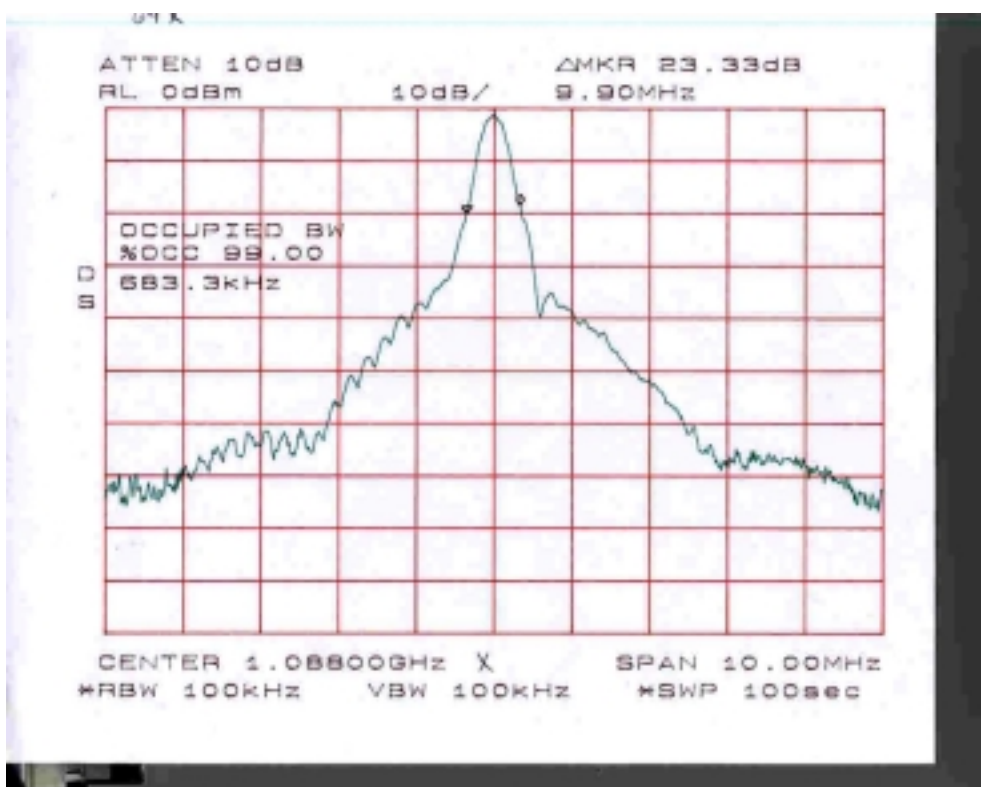
Figure 15 Pulse Spectrum of channel 64X showing 99% occupied bandwidth
