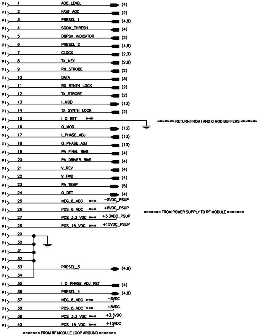
A2P1 BASED ON RF SCHEMATIC PIN INTERCONNECTS
