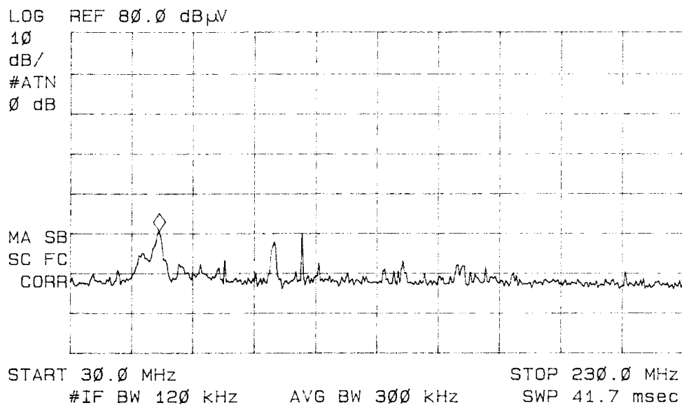
Figure 1 Radiated Emissions taken in screen room.
