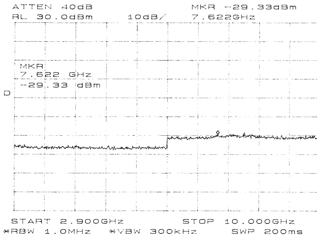
Figure 4 Emissions at Antenna Terminal
