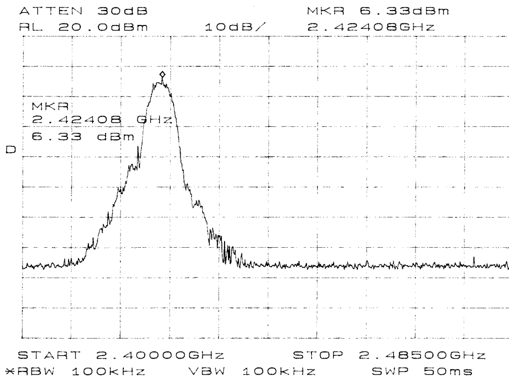
Figure 10 Emissions @ Antenna Port
