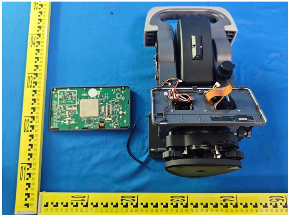
BT &amp; 2.4G WIFI &amp; 5G WIFI ANT
