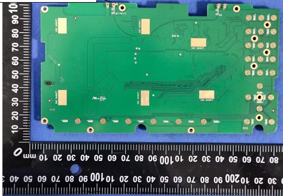
BT and WIFI ANT interface
