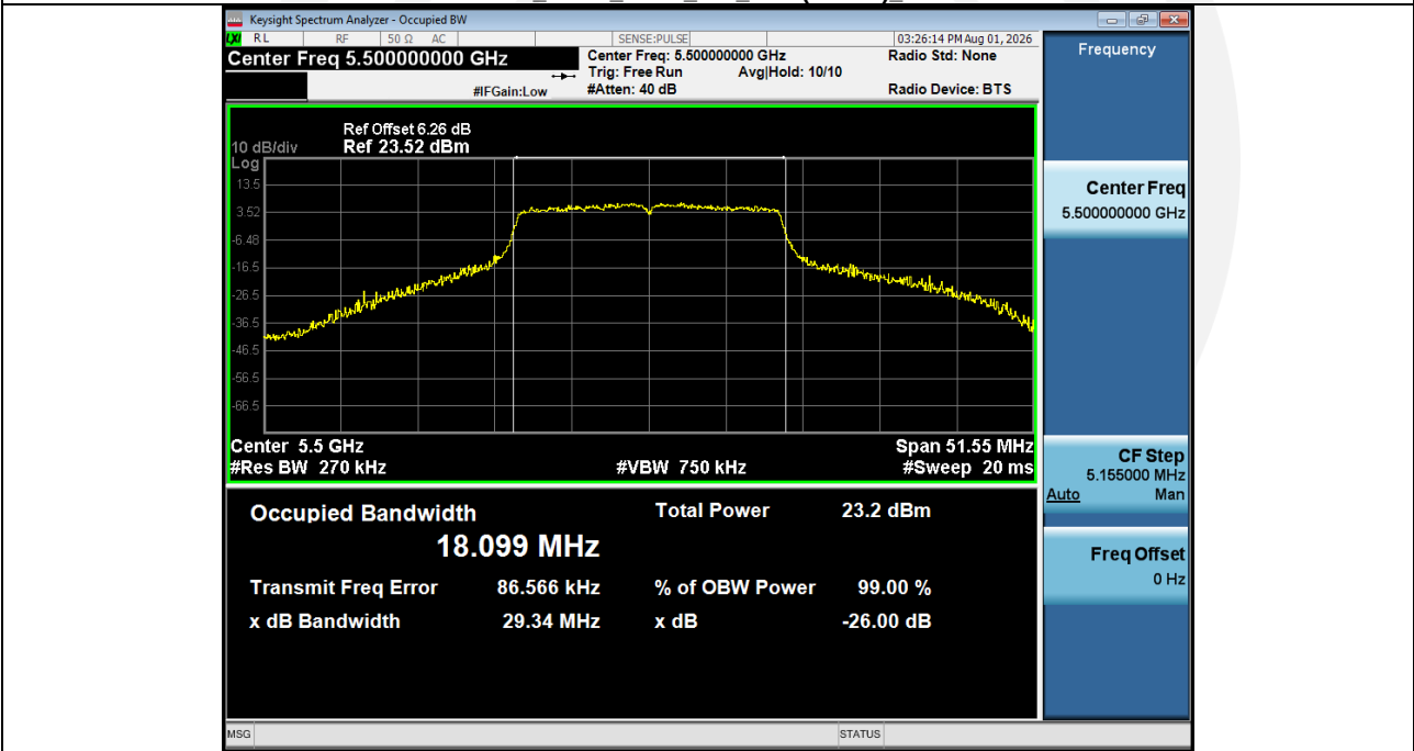
-26BW_NVNT_ANT1_802_11ac(VHT20)_5500
