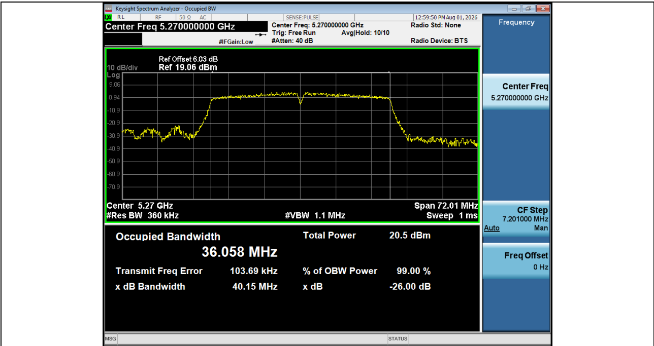
-26BW_NVNT_ANT1_802_11ac(VHT40)_5270
