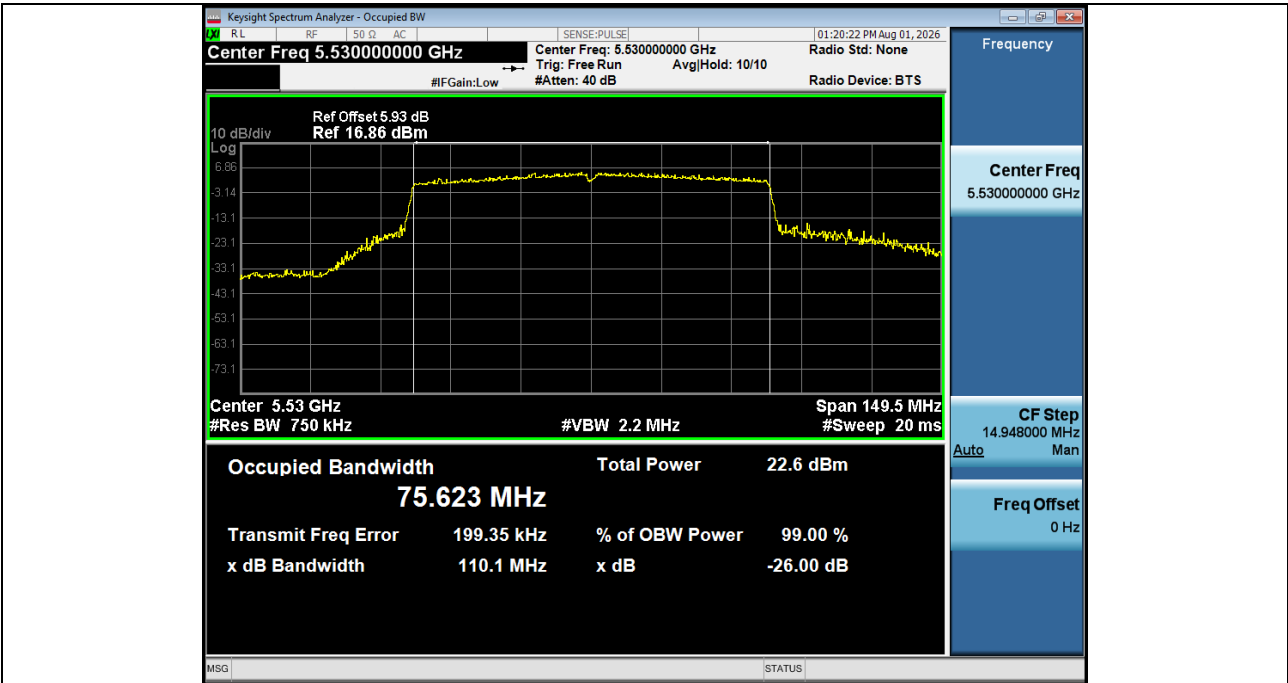
-26BW_NVNT_ANT1_802_11ac(VHT80)_5530
