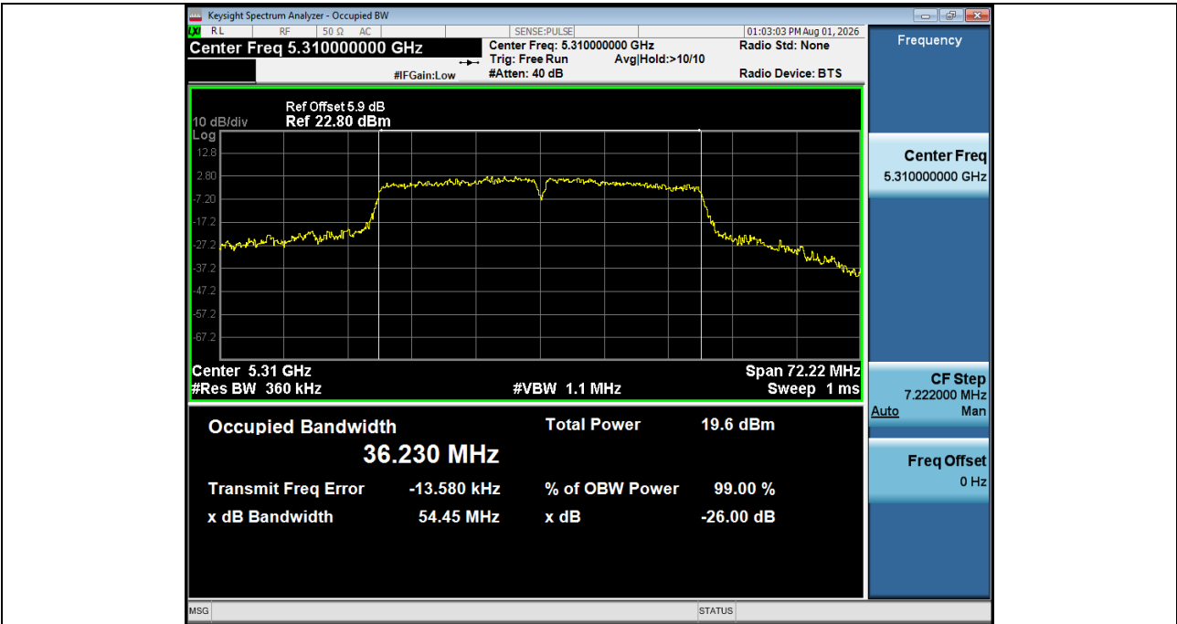
-26BW_NVNT_ANT1_802_11ac(VHT40)_5310
