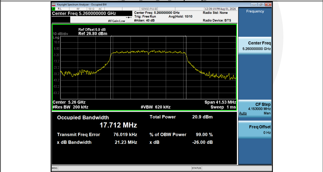
-26BW_NVNT_ANT1_802_11ac(VHT20)_5260
