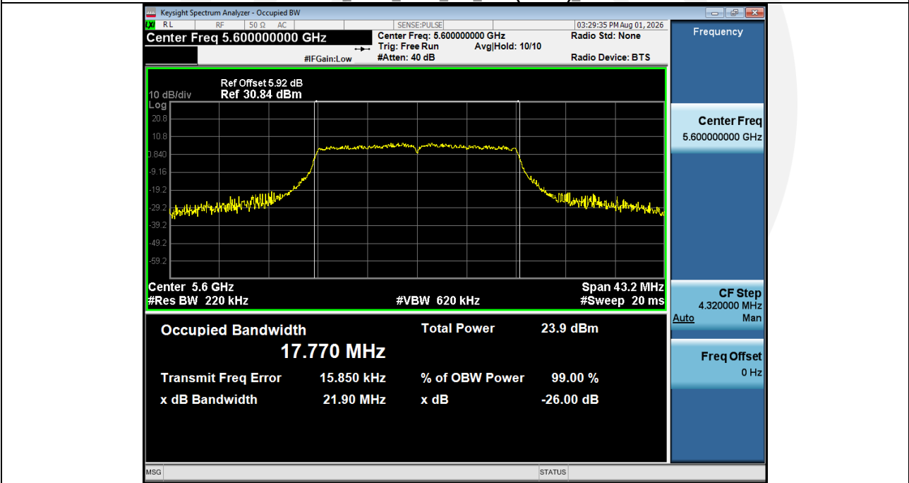
-26BW_NVNT_ANT1_802_11ac(VHT20)_5600
