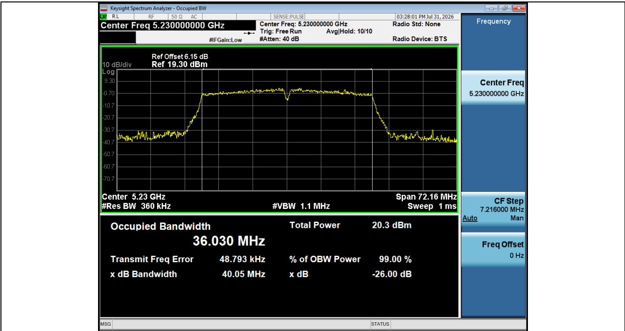
-26BW_NVNT_ANT1_802_11ac(VHT40)_5230
