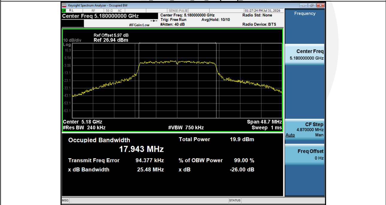
-26BW_NVNT_ANT1_802_11n(HT20)_5180
