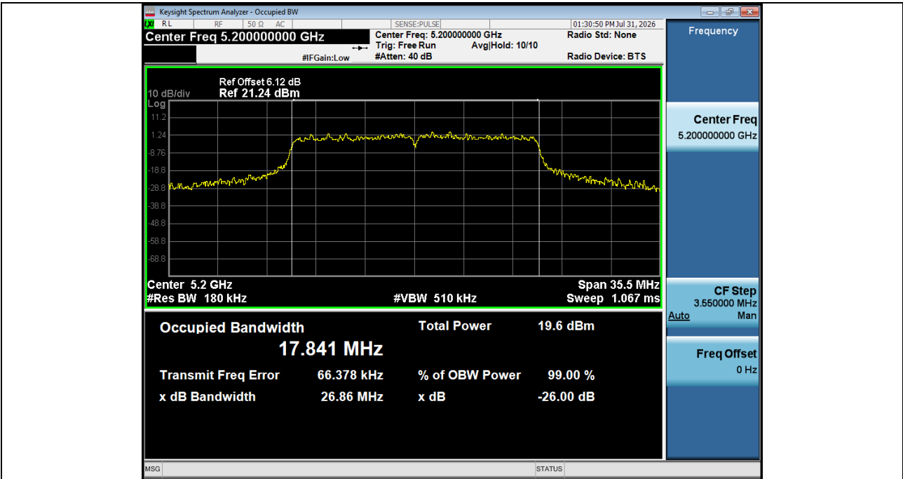
-26BW_NVNT_ANT1_802_11n(HT20)_5200
