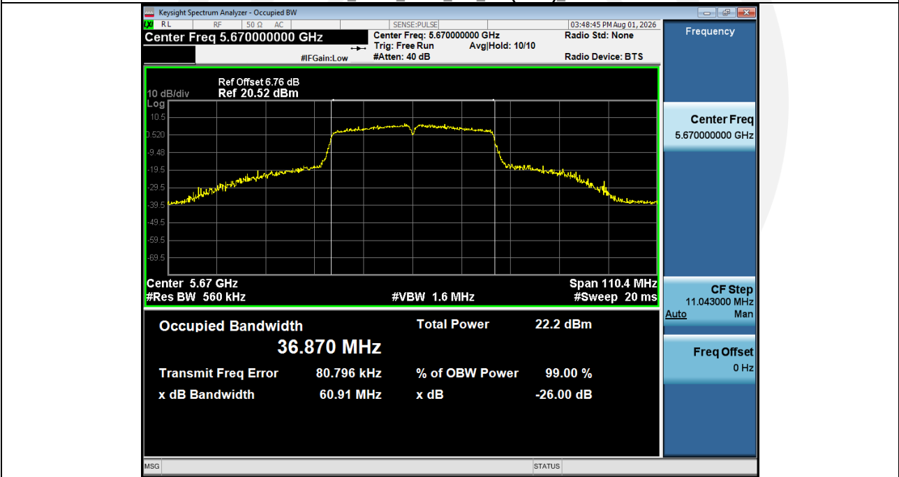
-26BW_NVNT_ANT1_802_11n(HT40)_5670
