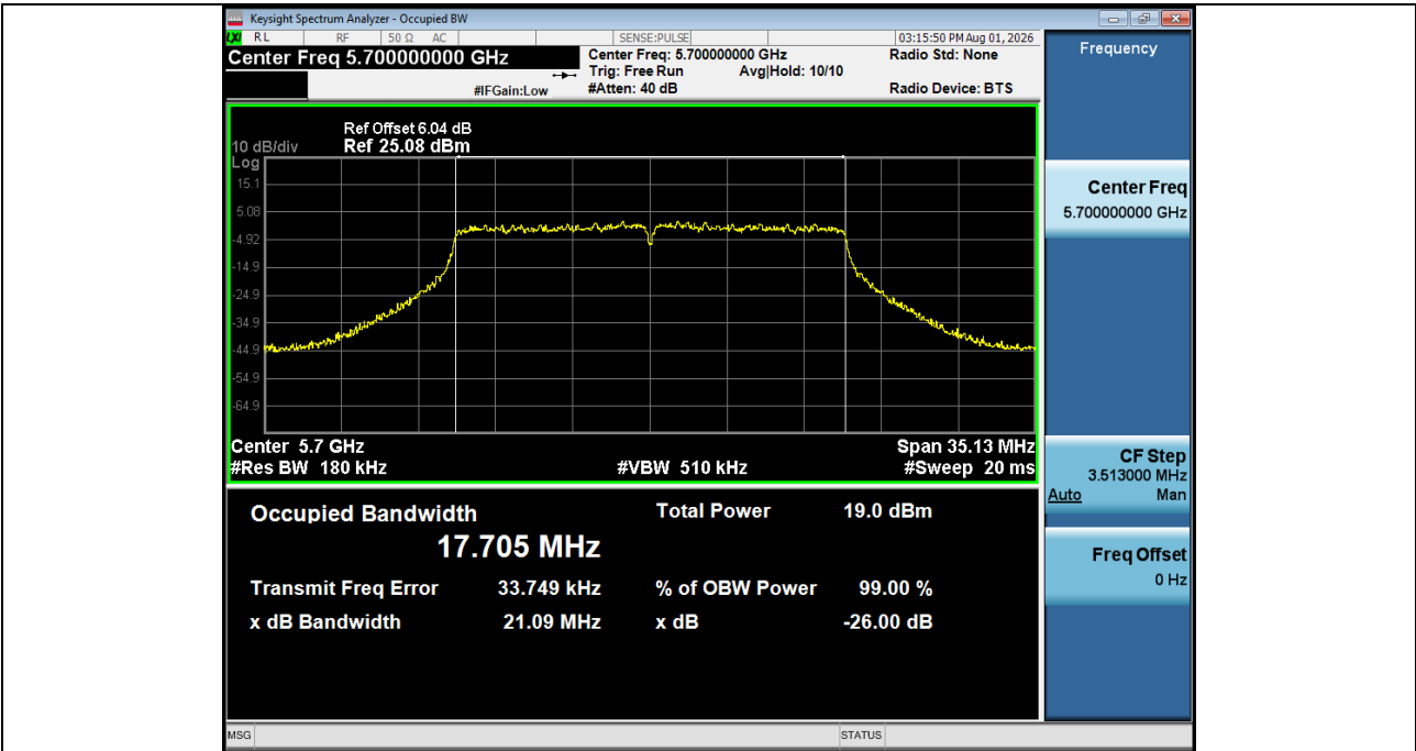
-26BW_NVNT_ANT1_802_11n(HT20)_5700
