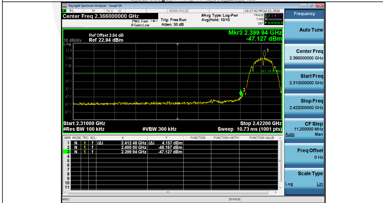
2 Bandedge_NVNT_ANT1_802_11b_2412
