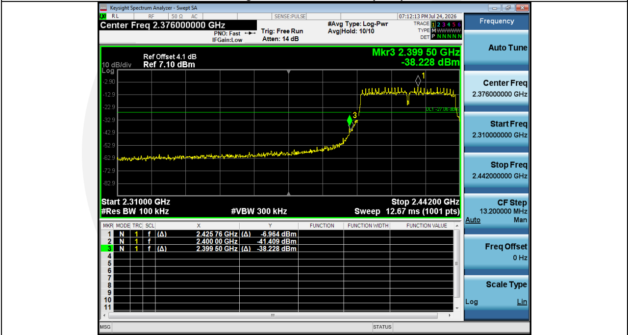
2. Bandedge NVNT_ANT1_802_11n(HT40)_2422
