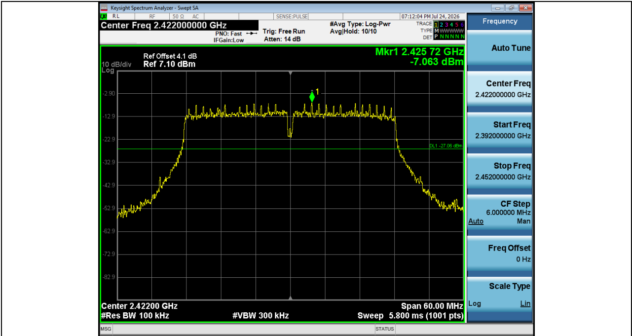
2. Bandedge NVNT_ANT1_802_11n(HT40)_2422
