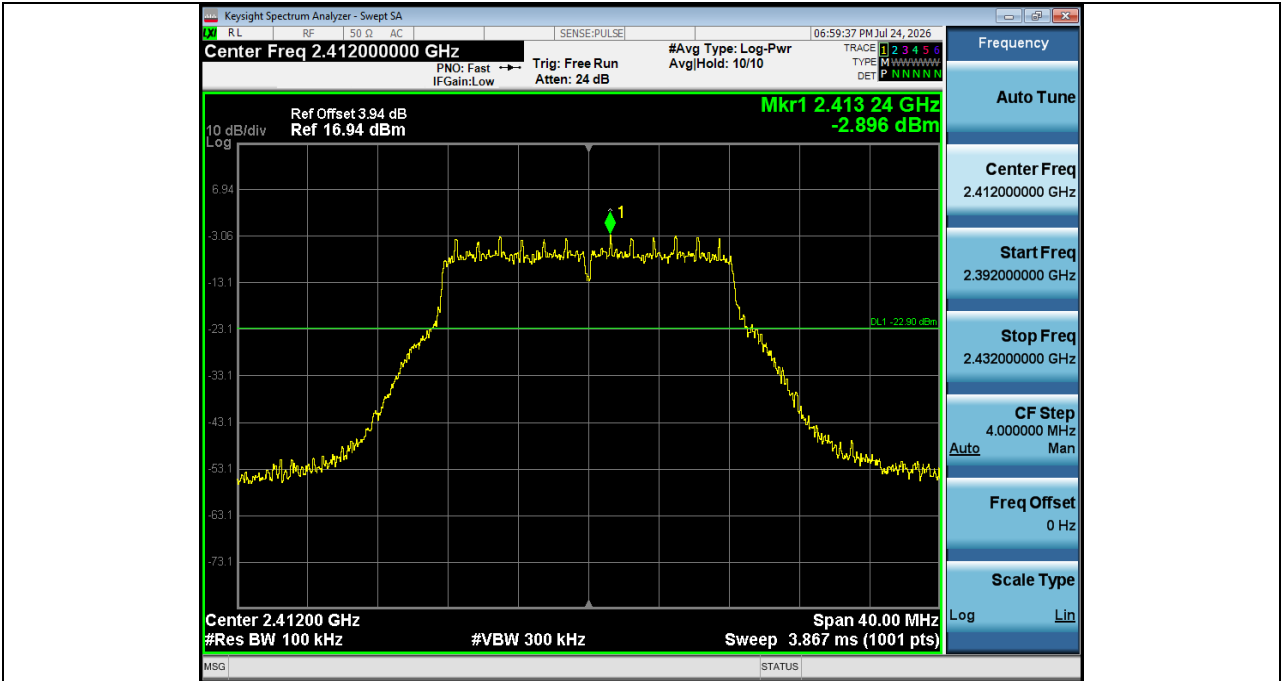
2. Spurious Emission NVNT_ANT1_802_11g_2412
