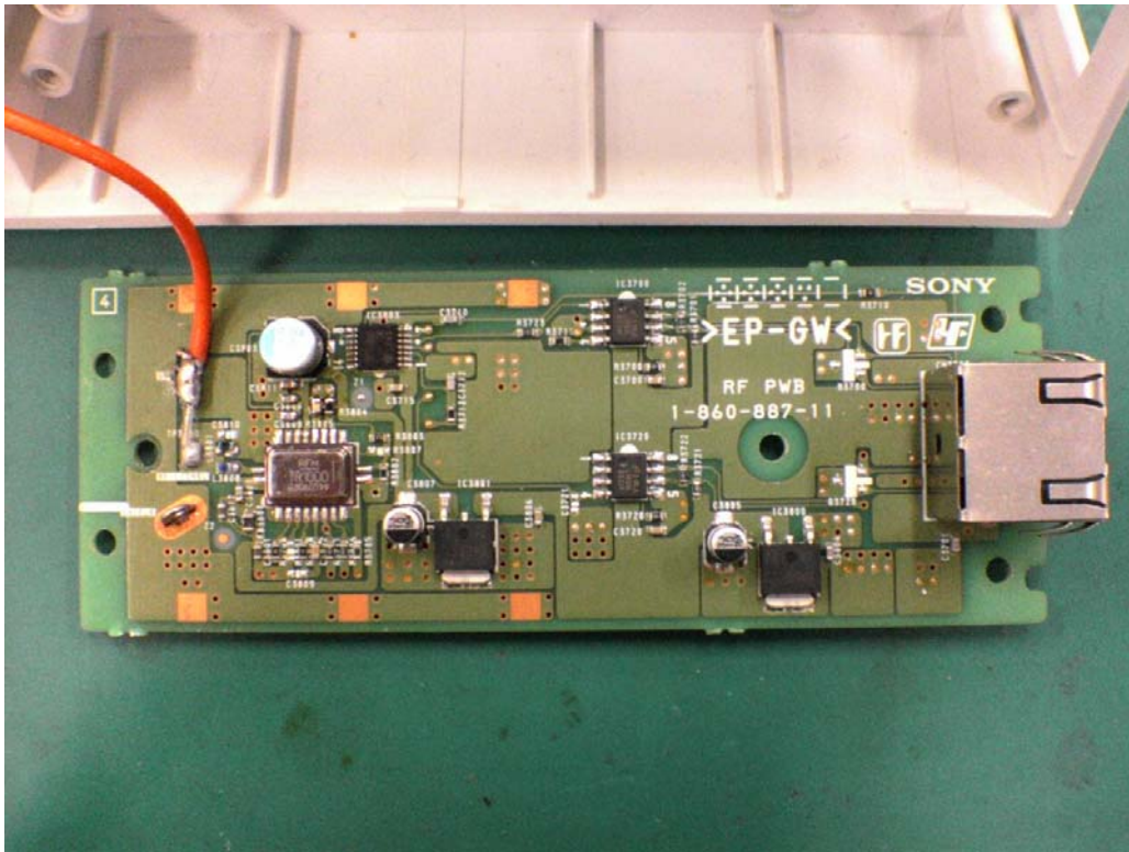
front (RF Module)
