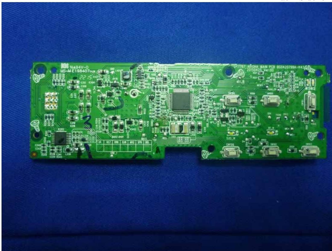
Figure 2 Back Side of PCB Board
