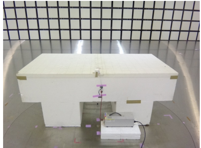
30 - 1000 MHz
