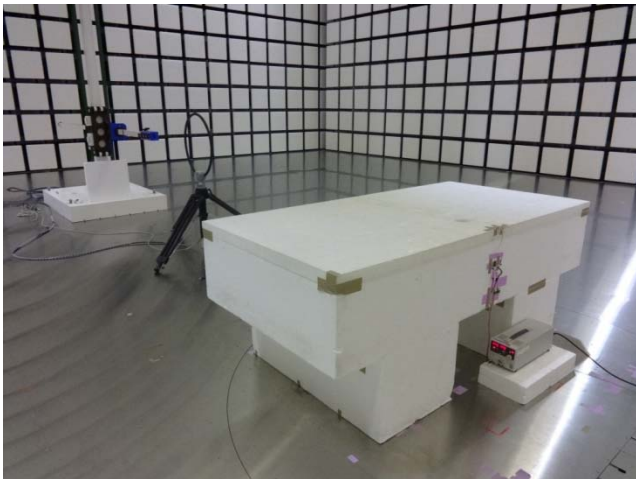
Below 30MHz
