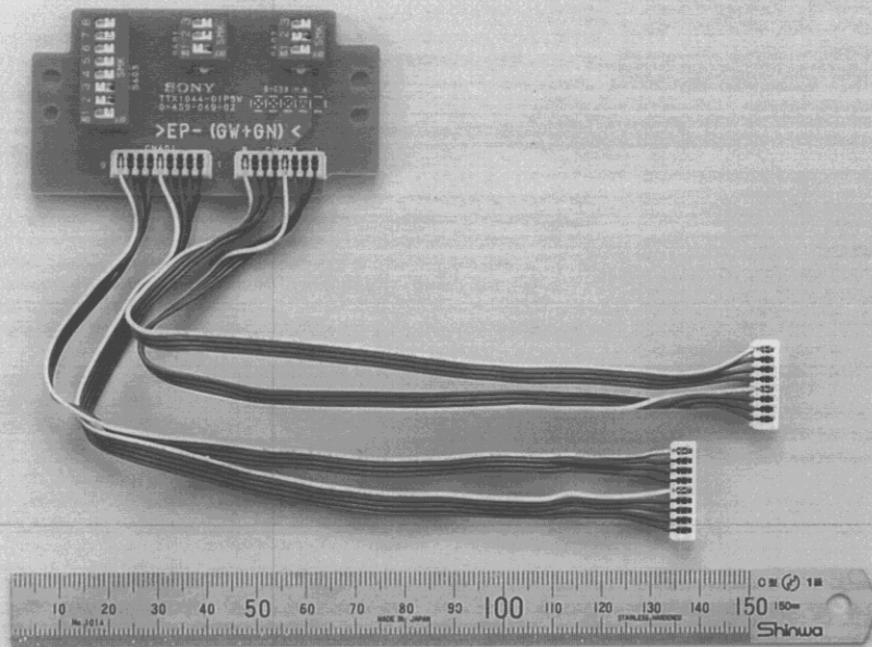
CDL1100-40 : DIP SW P.C.Board, Side A View
