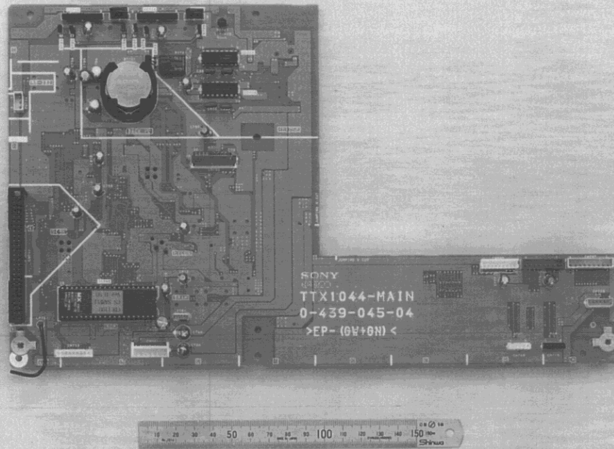
CDL1100-40 : MAIN P.C.Board, Side A View
