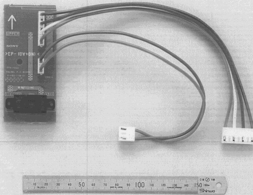
CDL1100-40 : VOLSEL P.C.Board, Side A View
