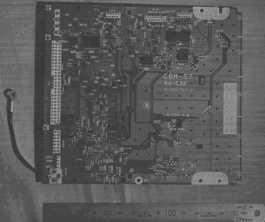
CDL1100-40 : CDM-57(CD-ROM DRIVE UNIT) ; MA-C30 P.C.Board, Side B View
