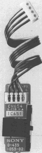
FG SENSOR P.C.Board
