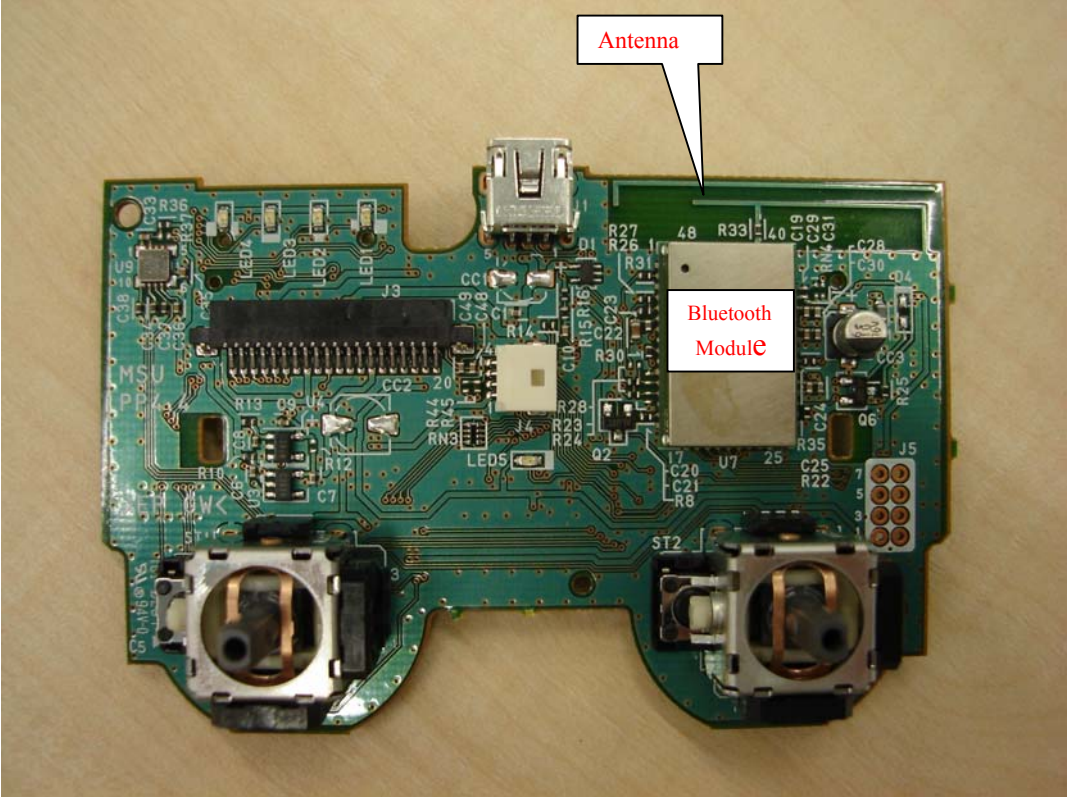
View 3 Location of Antenna & Module
