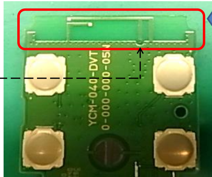
Bluetooth Antenna
