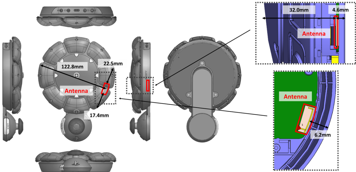
Antenna position
