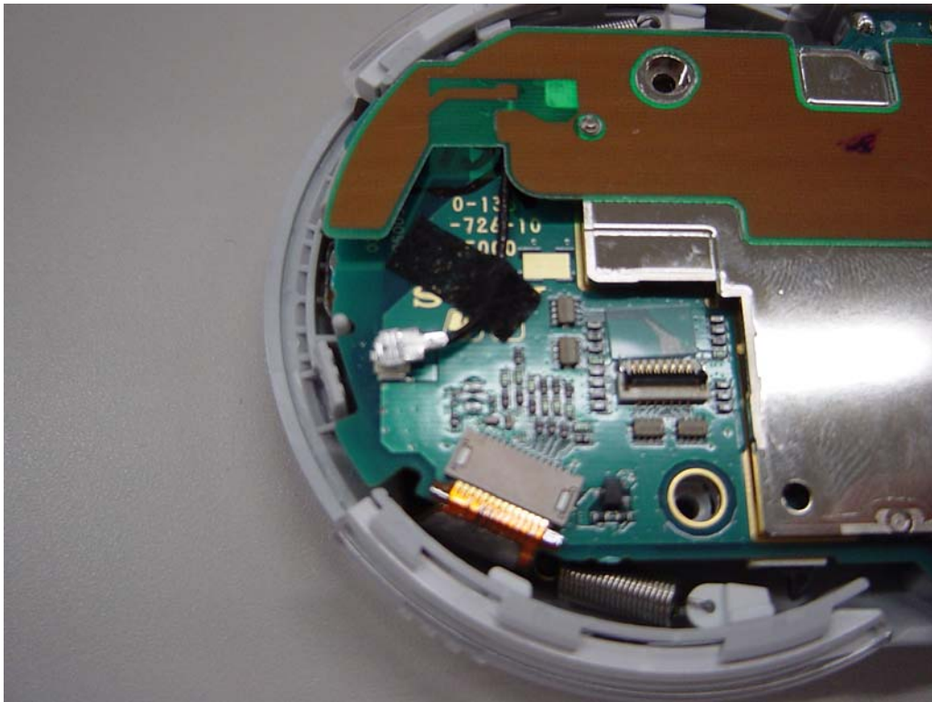
Antenna 3
