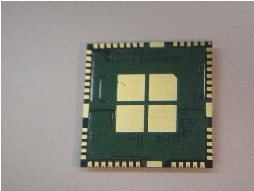
RF Module (Rear)
