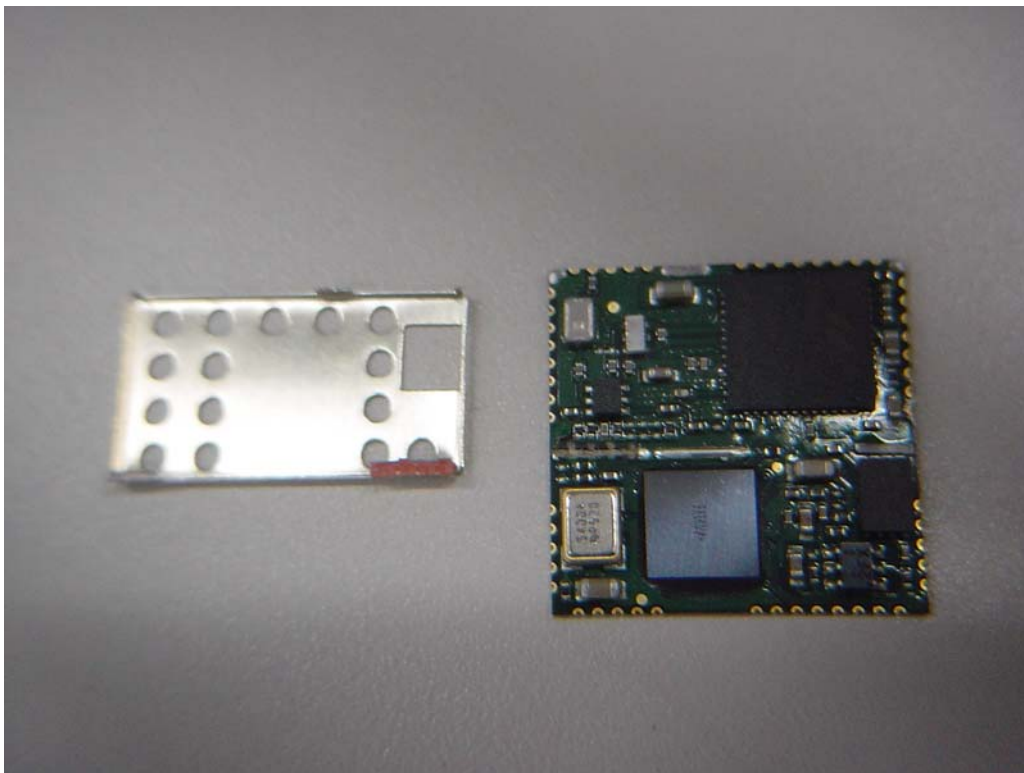
RF Module without Shield 1 (Front)
